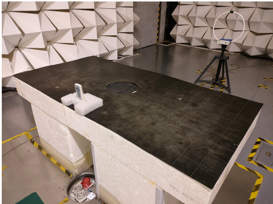
Model: RF25 For 9kHz-30MHz Test Site 2#
