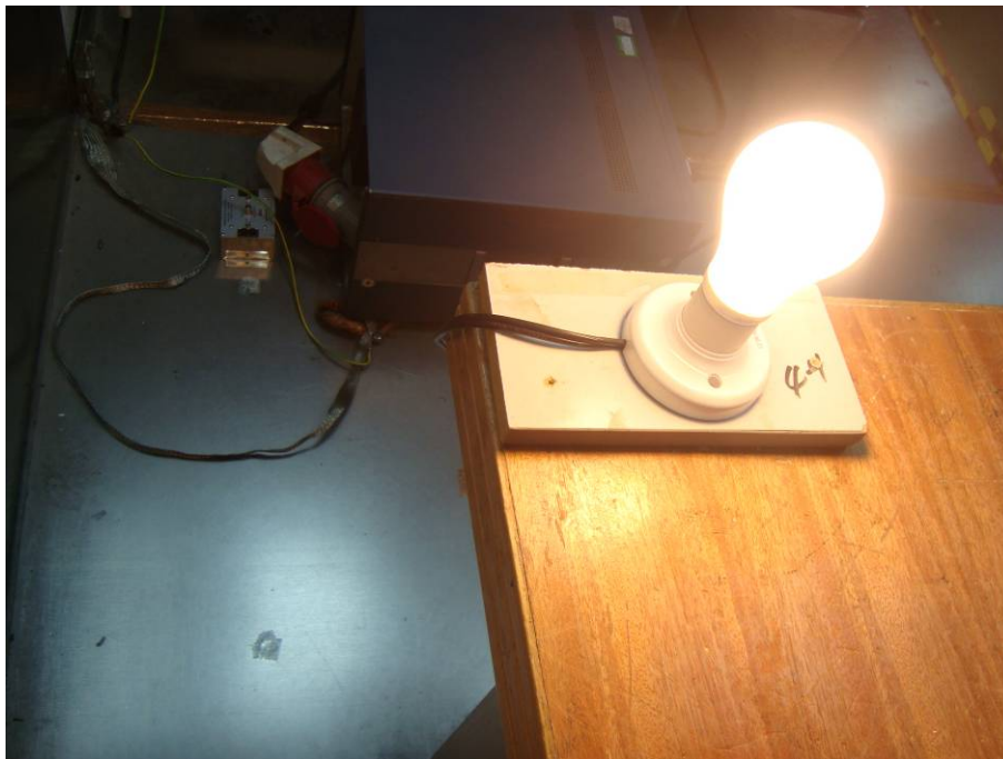
Conduction Emissions - Side View (Model: EBA-28 20W)
