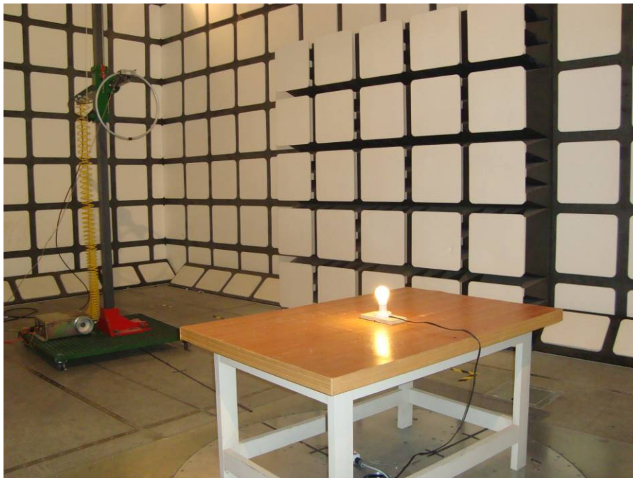
Radiated Emissions - Rear View (Model: EBA-28 15W)
