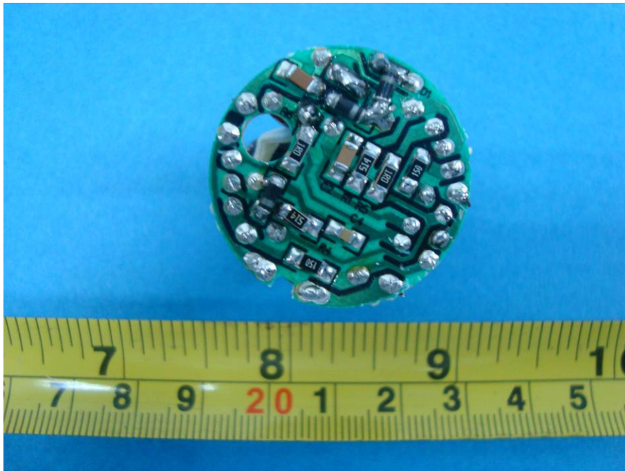
EUT – Mainboard Bottom View (Model: EBA-28 20W)
