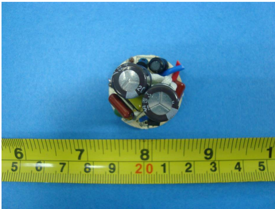
EUT – Mainboard Top View (Model: EBA-28 15W)
