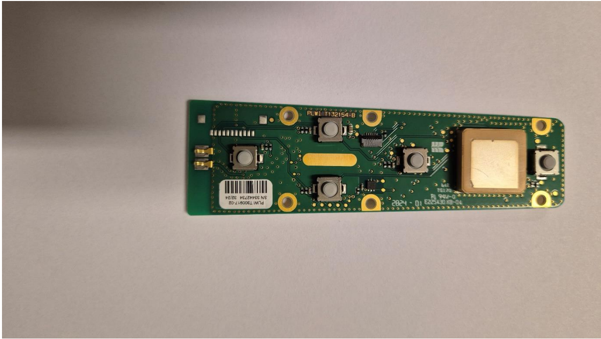
Figure 13 PLWI Radio board, primary side.
