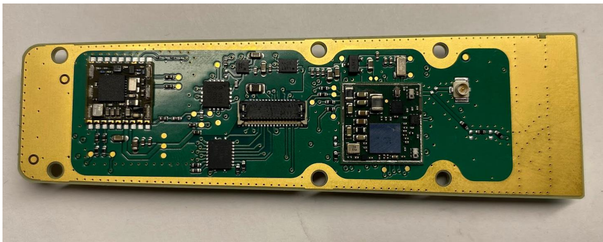
Figure 16 PLWI without shieldings
