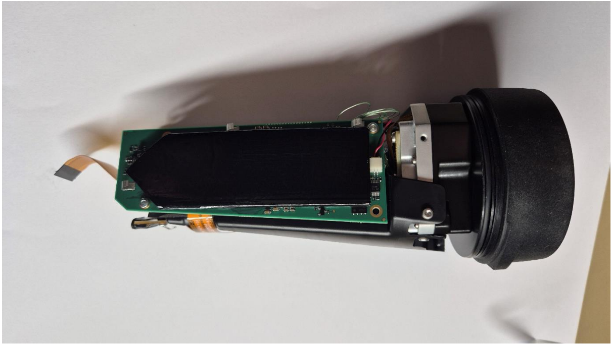
Figure 9 FLIR-O1500, Housing removed. CPU side.
