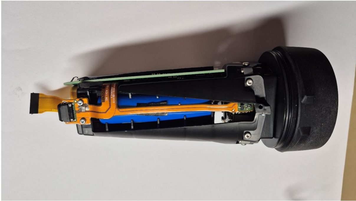
Figure 11 FLIR-O1500, Bottom side with USB connector.
