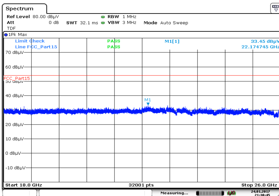
Plot 11: 18 GHz to 26 GHz, 5200 MHz, vertical & horizontal polarization
