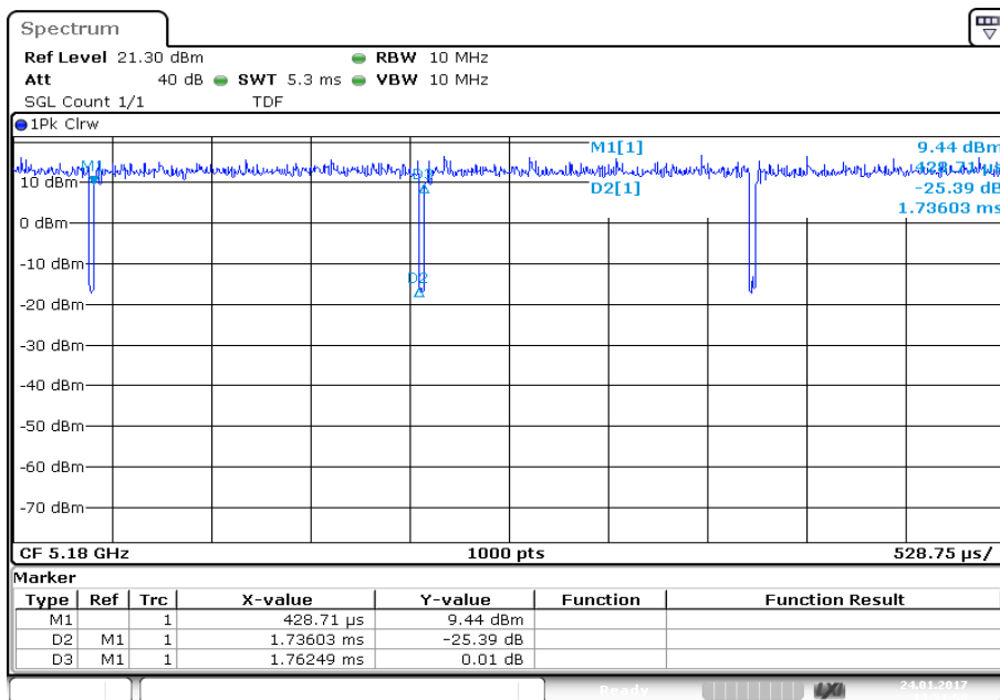
Plot 2: duty cycle of the transmitter – OFDM / n HT20 – mode
