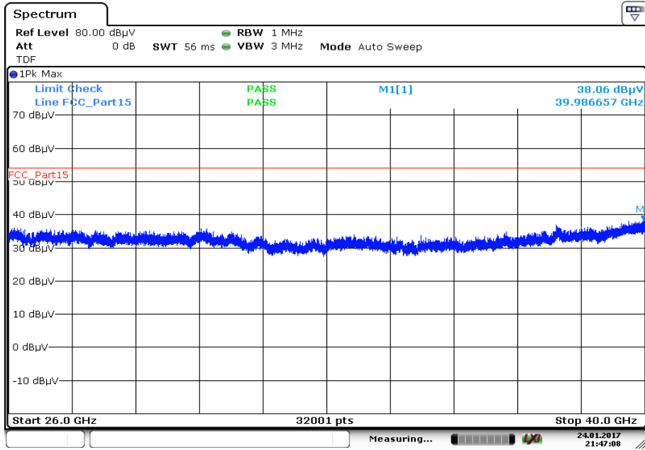
Plot 12: 26 GHz to 40 GHz, 5200 MHz, vertical & horizontal polarization
