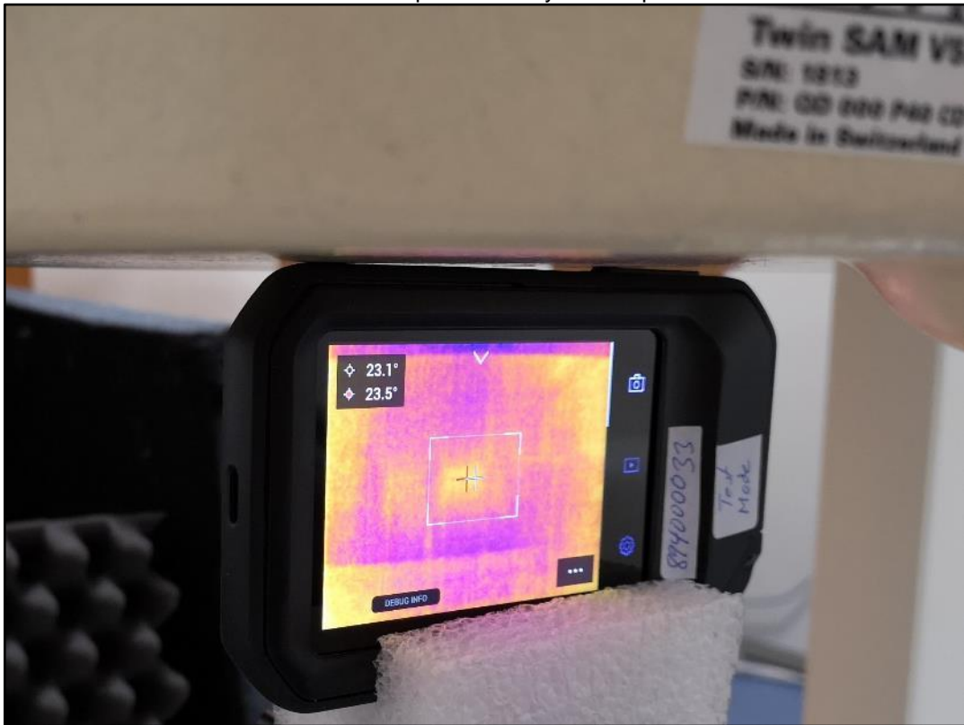
Photo 8: Test position body worn bottom side
