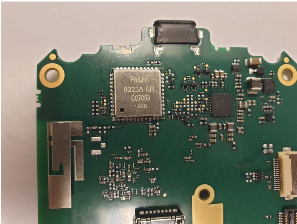
Figure 8 Radio module Fn-Link 8223A-SR and antenna.
