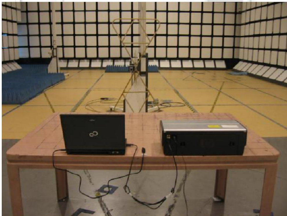
Receiver Radiated Emissions Test Setup (Rear View)
