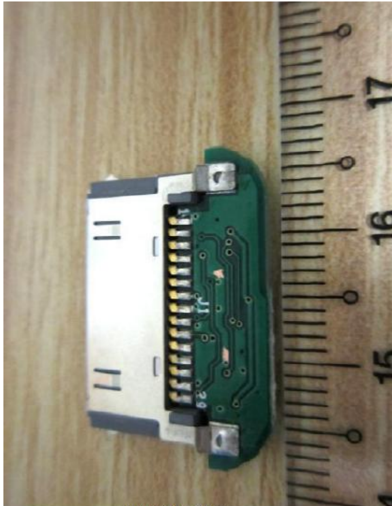
EUT PCB Trace Side
