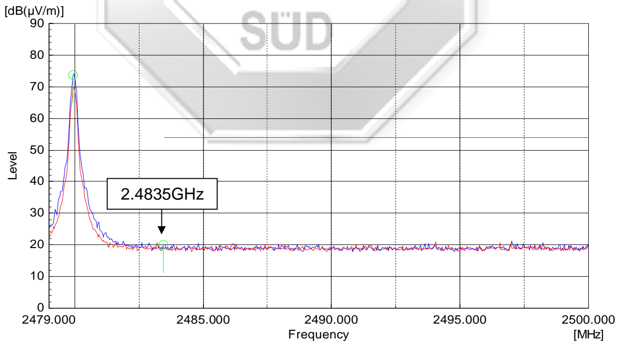
Plot 34 – Upper Band Edge at 2.4835GHz
