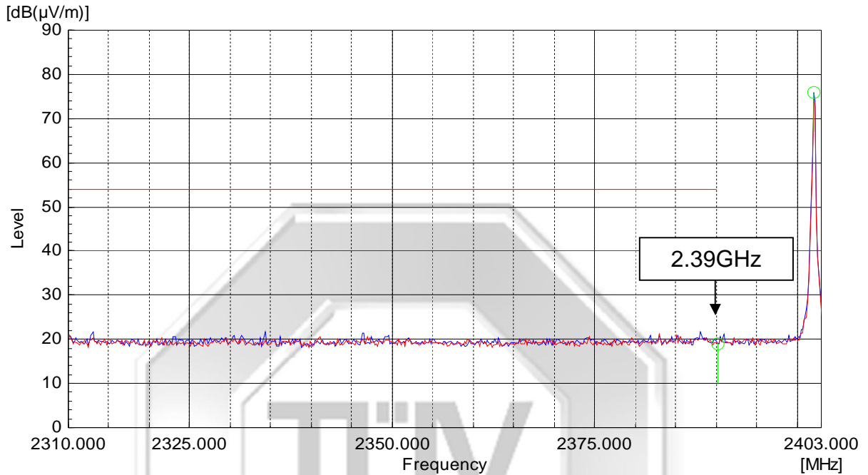
Plot 33 – Lower Band Edge at 2.4000GHz
