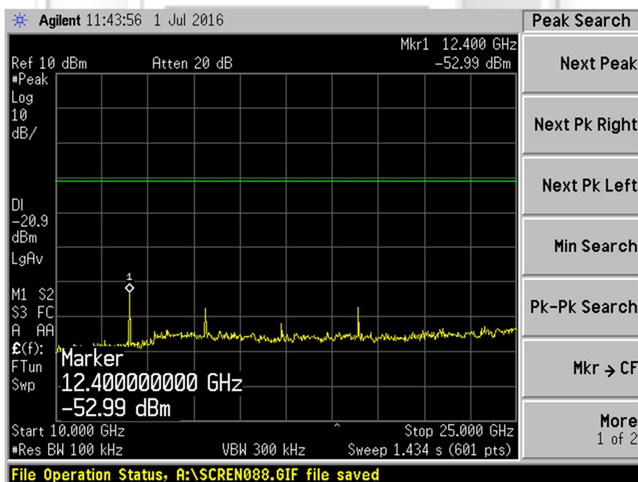
Plot 12 – Channel 39 (upper ch)
