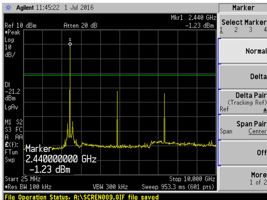
Plot 9 – Channel 19 (middle ch)
