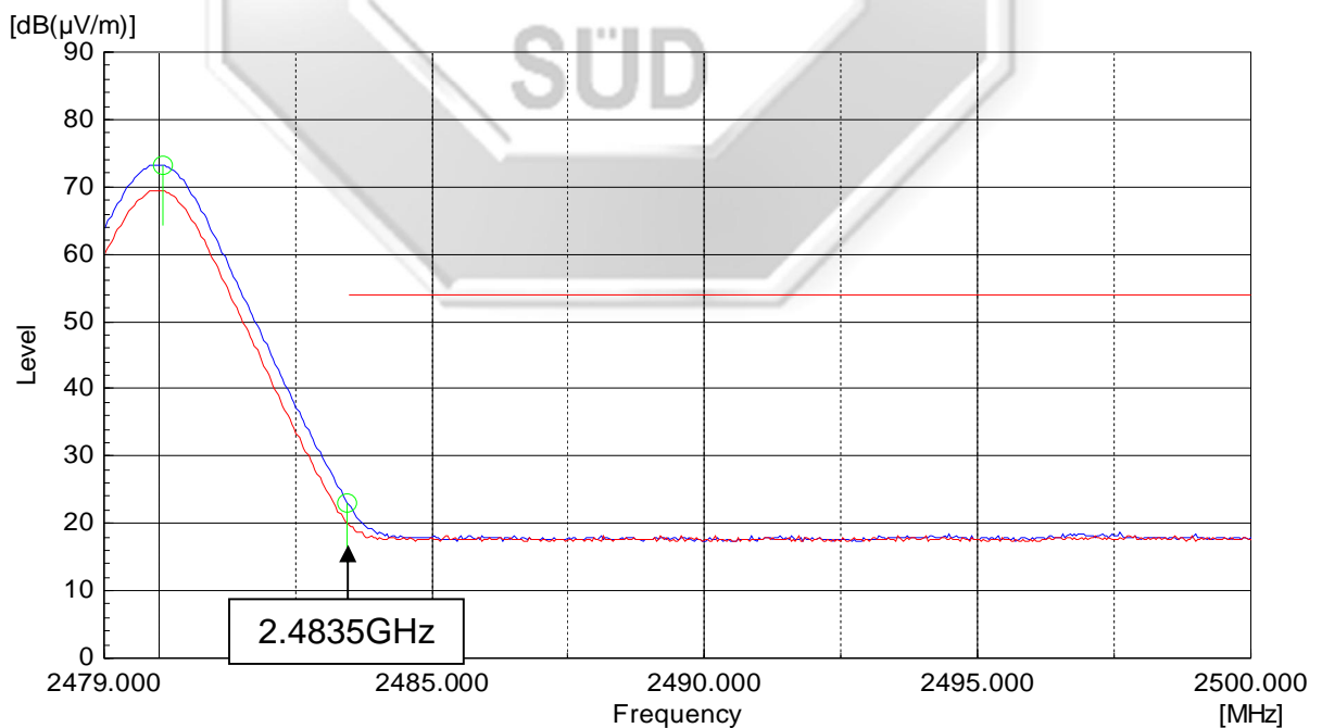
Plot 38 – Average Plot at Upper Band Edge at 2.4835GHz
