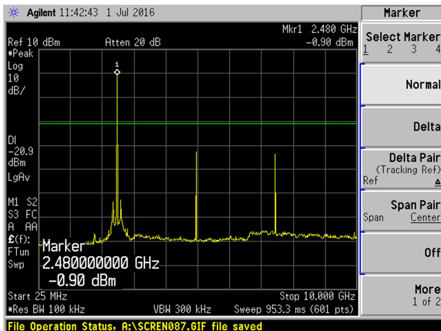
Plot 11 – Channel 39 (upper ch)
