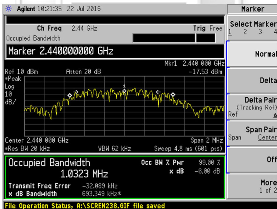
Plot 5 - Channel 19 (middle ch)
