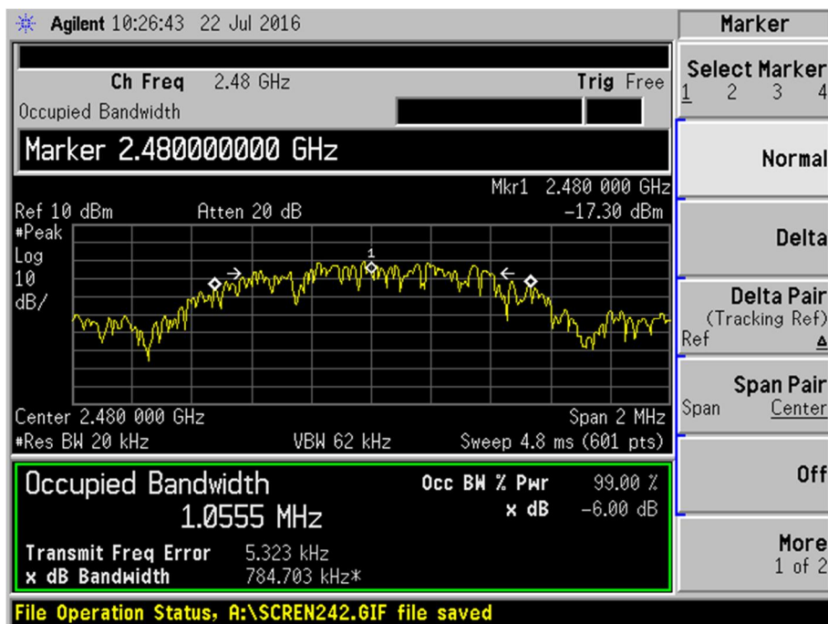
Plot 6 - Channel 39 (upper ch)
