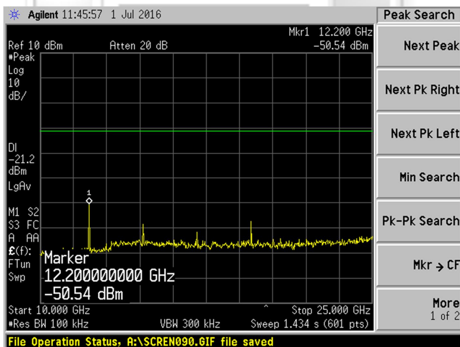
Plot 10 – Channel 19 (middle ch)
