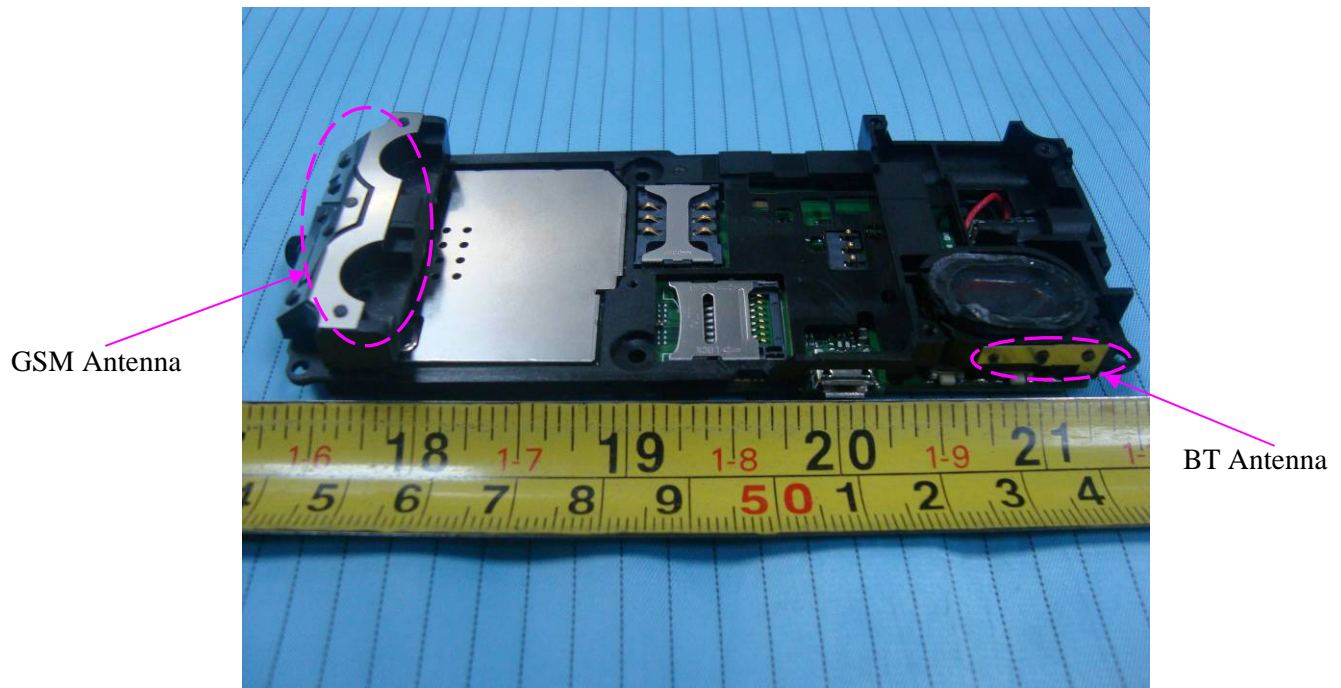
EUT – Main Board Cover off View
