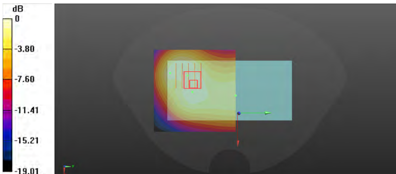
0 dB = 0.819 W/kg
