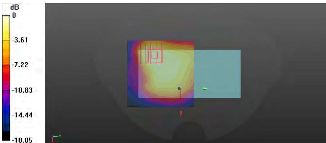
0 dB = 0.358 W/kg
