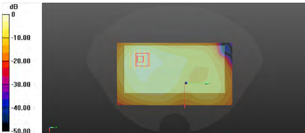
0 dB = 0.312 W/kg
