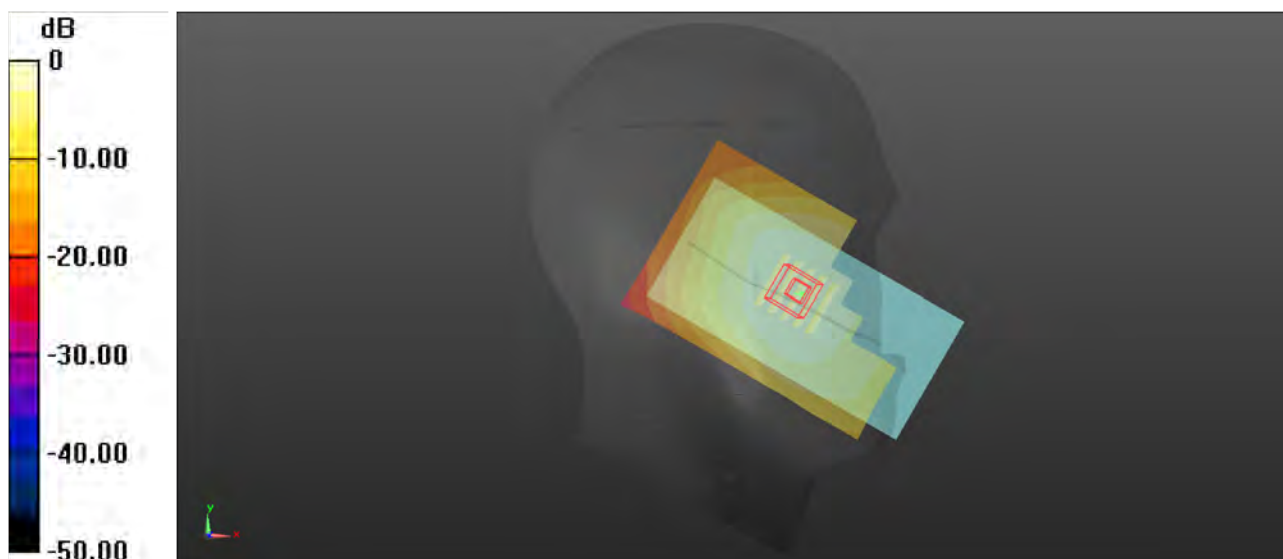
0 dB = 0.681 W/kg
