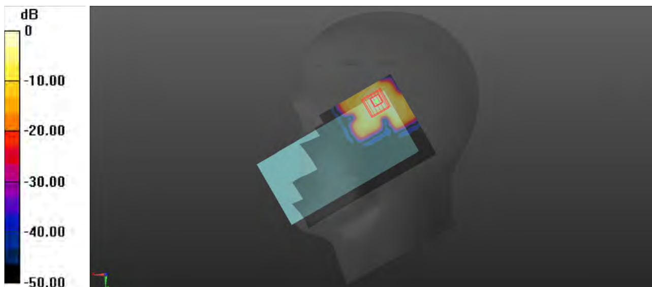
0 dB = 0.685 W/kg
