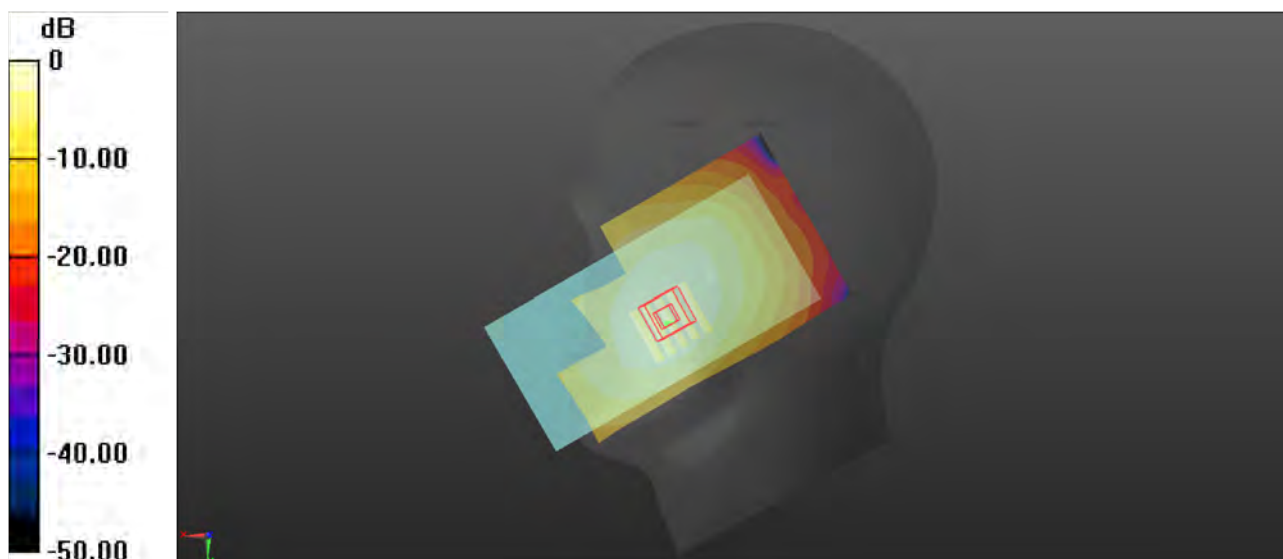
0 dB = 0.418 W/kg
