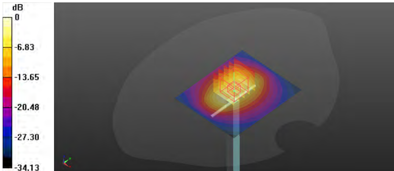
0 dB = 12.6 W/kg
