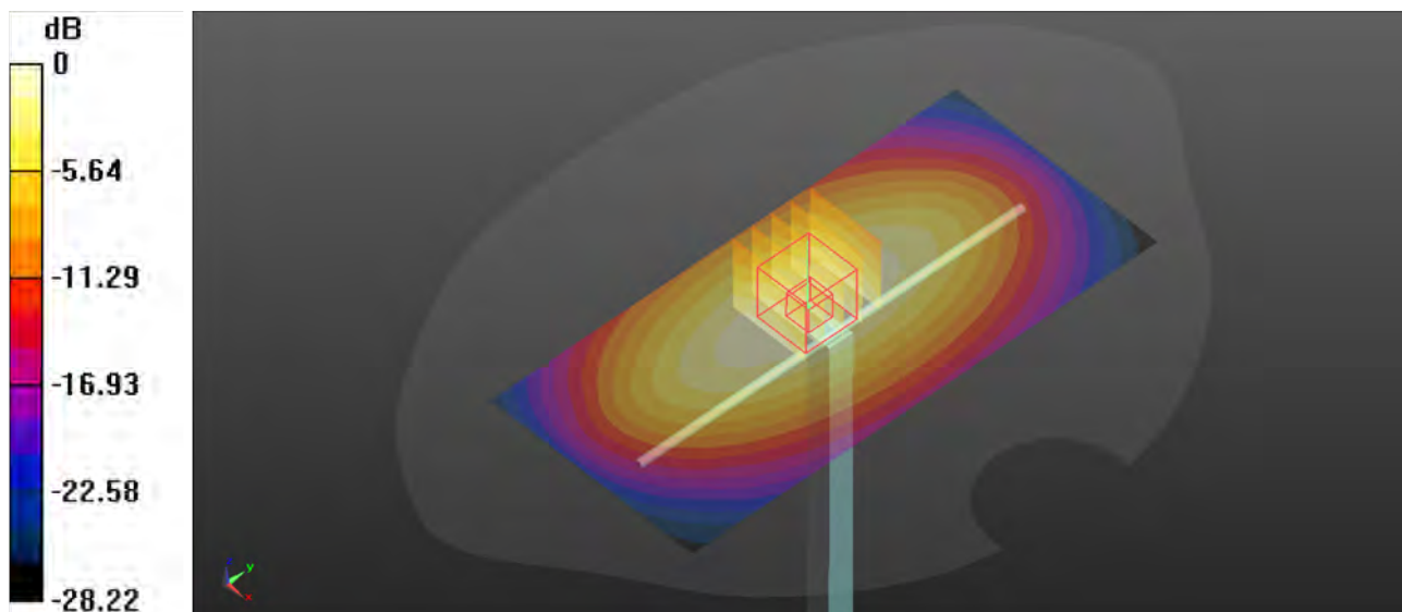
0 dB = 2.52 W/kg
