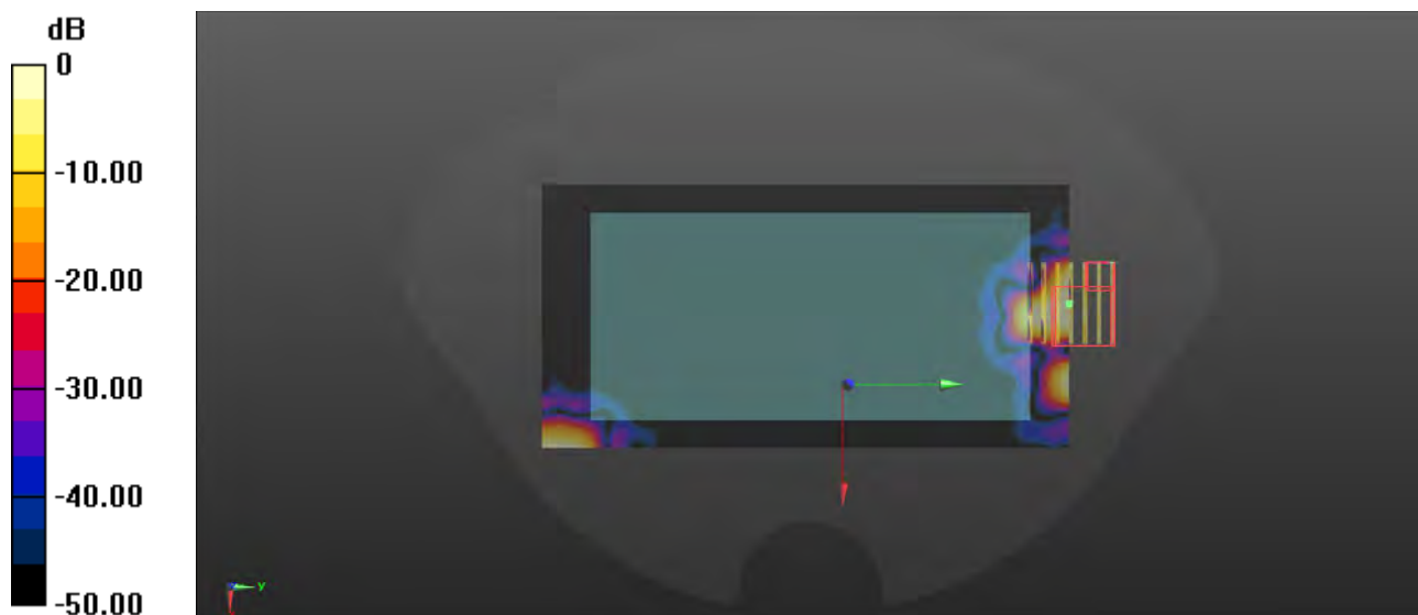
0 dB = 0.00227 W/kg
