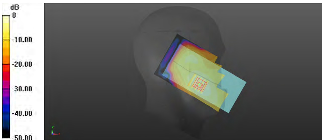
0 dB = 0.210 W/kg
