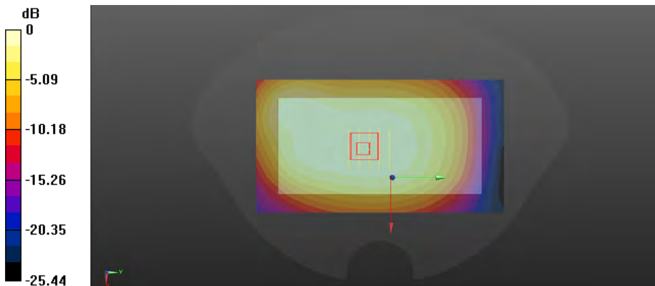
0 dB = 0.382 W/kg
