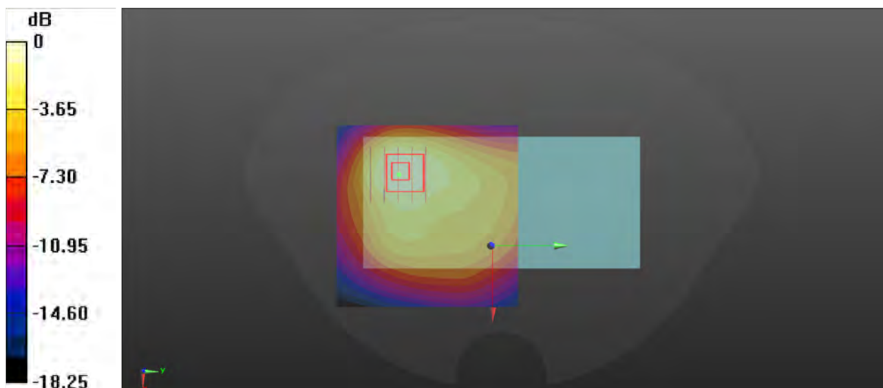
0 dB = 0.473 W/kg
