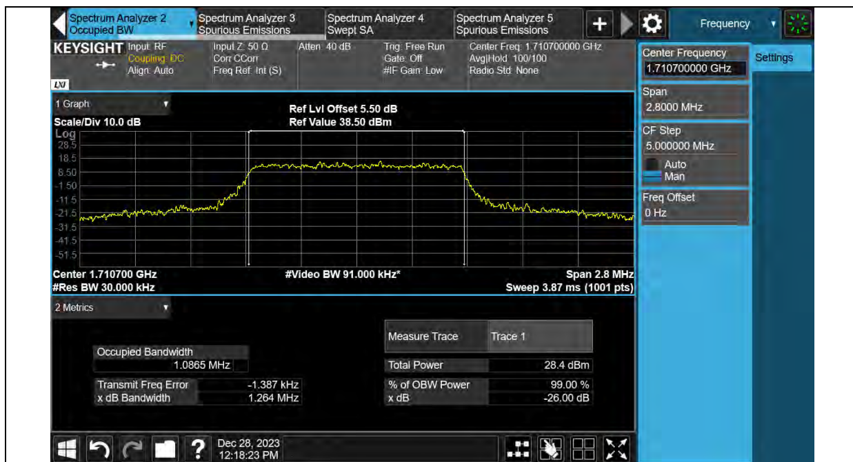
Band66-1.4MHz-64QAM-132322-6RB#0
