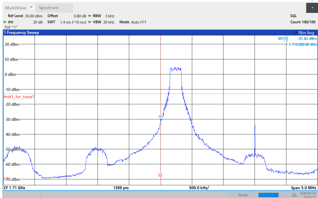
Band66-3MHz-16QAM-131987-15RB#0
