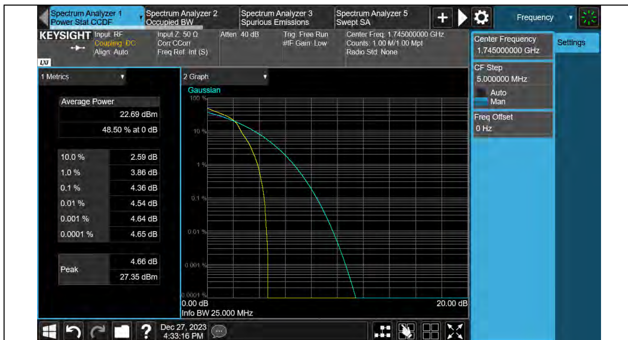
Band66-20MHz-16QAM-132322-100RB#0
