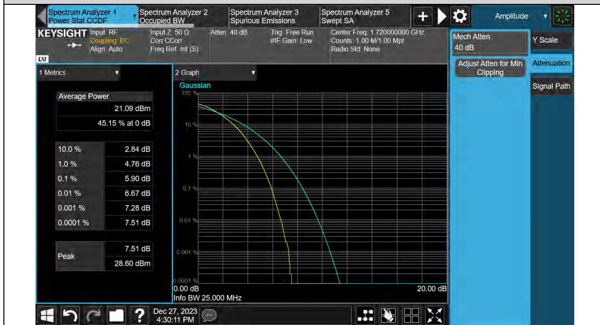
Band66-20MHz-64QAM-132322-1RB#0
