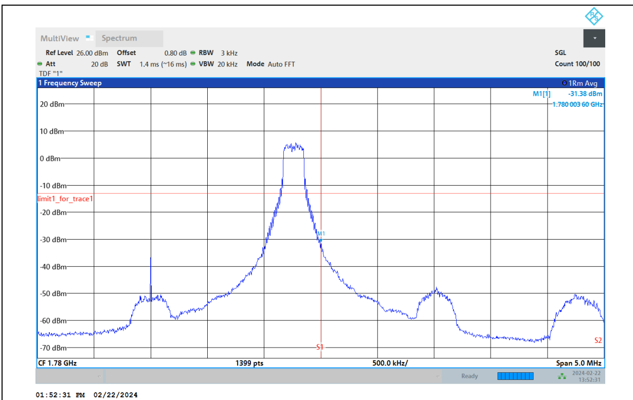
Band66-3MHz-16QAM-132657-15RB#0
