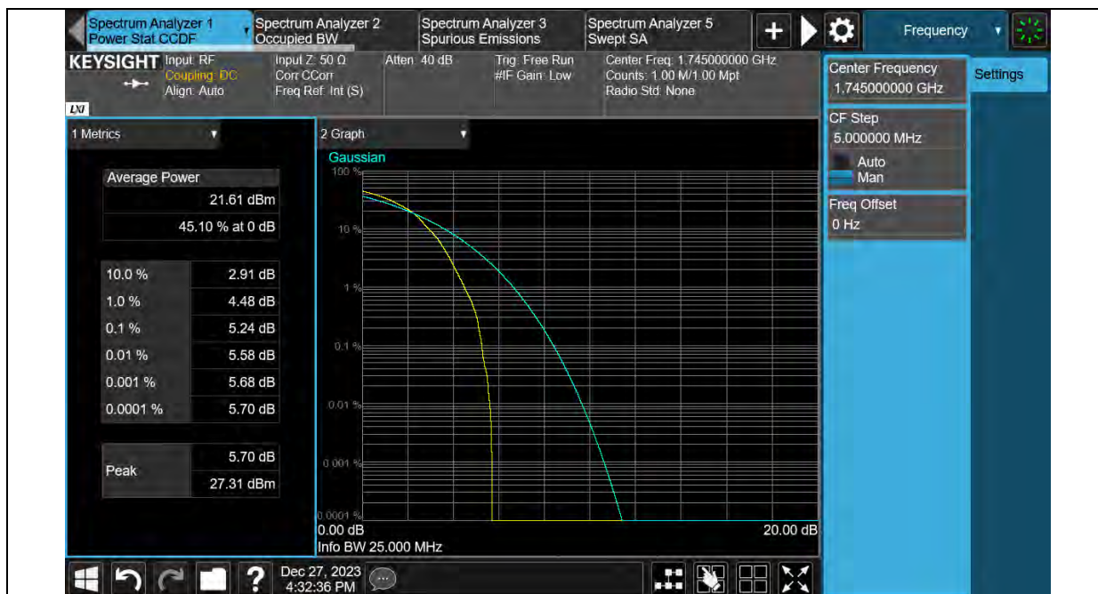
Band66-20MHz-64QAM-132322-100RB#0
