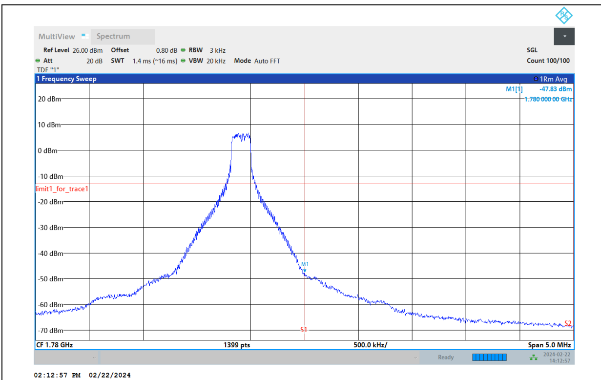
Band66-10MHz-QPSK-132622-50RB#0
