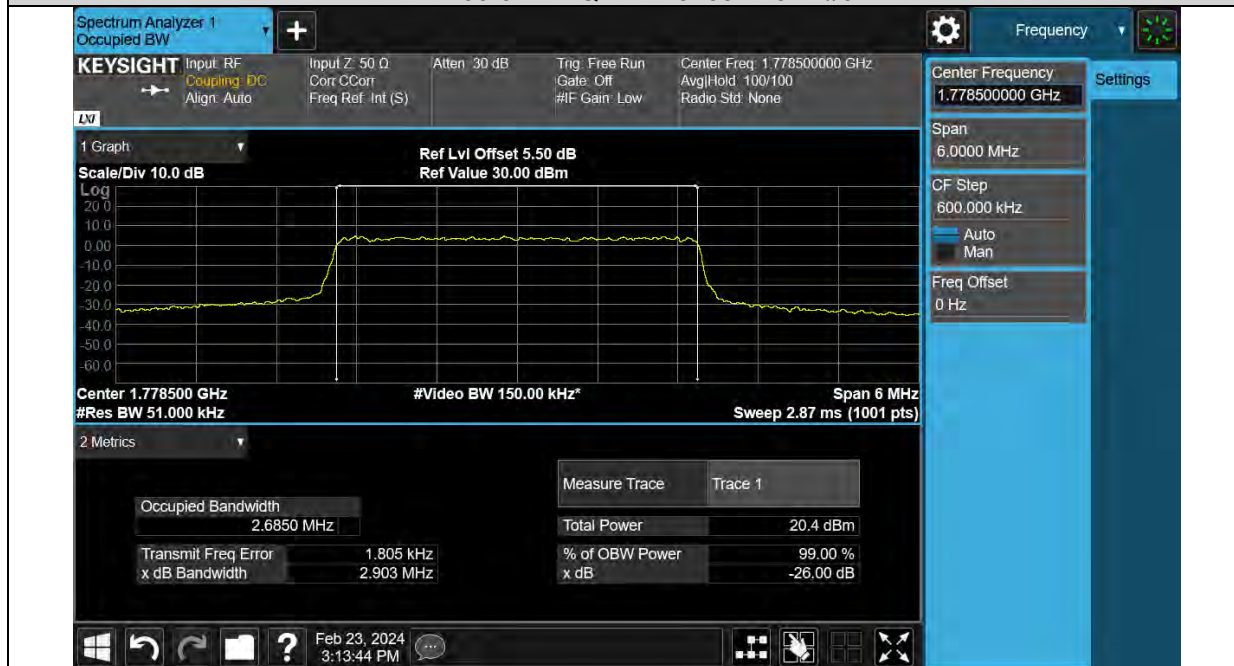
Band66-3MHz-16QAM-131987-15RB#0
