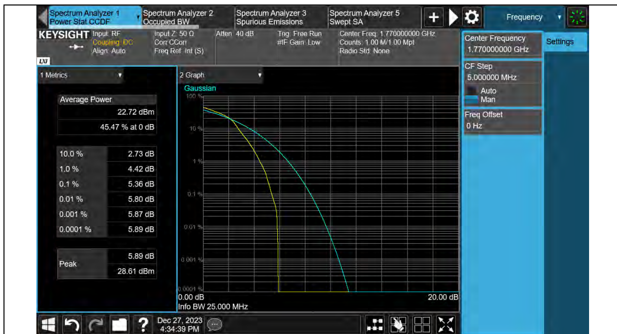
Band66-20MHz-16QAM-132572-100RB#0
