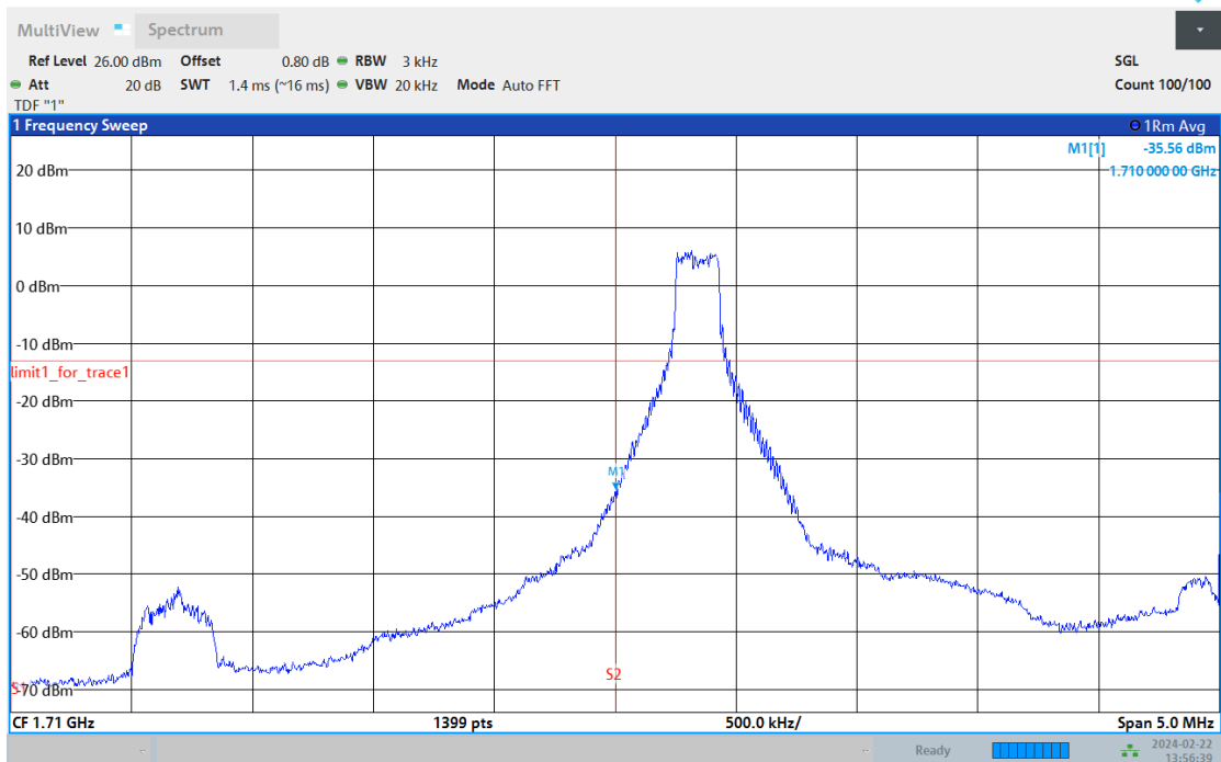
Band66-5MHz-QPSK-131997-25RB#0
