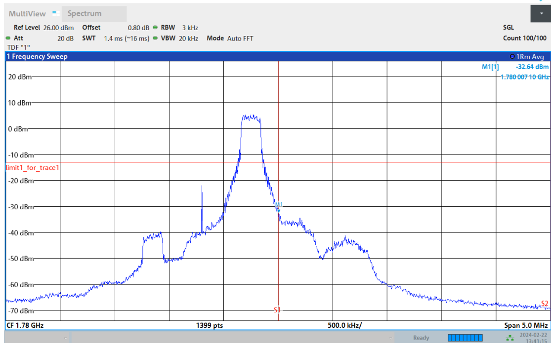
Band66-1.4MHz-16QAM-132665-6RB#0
