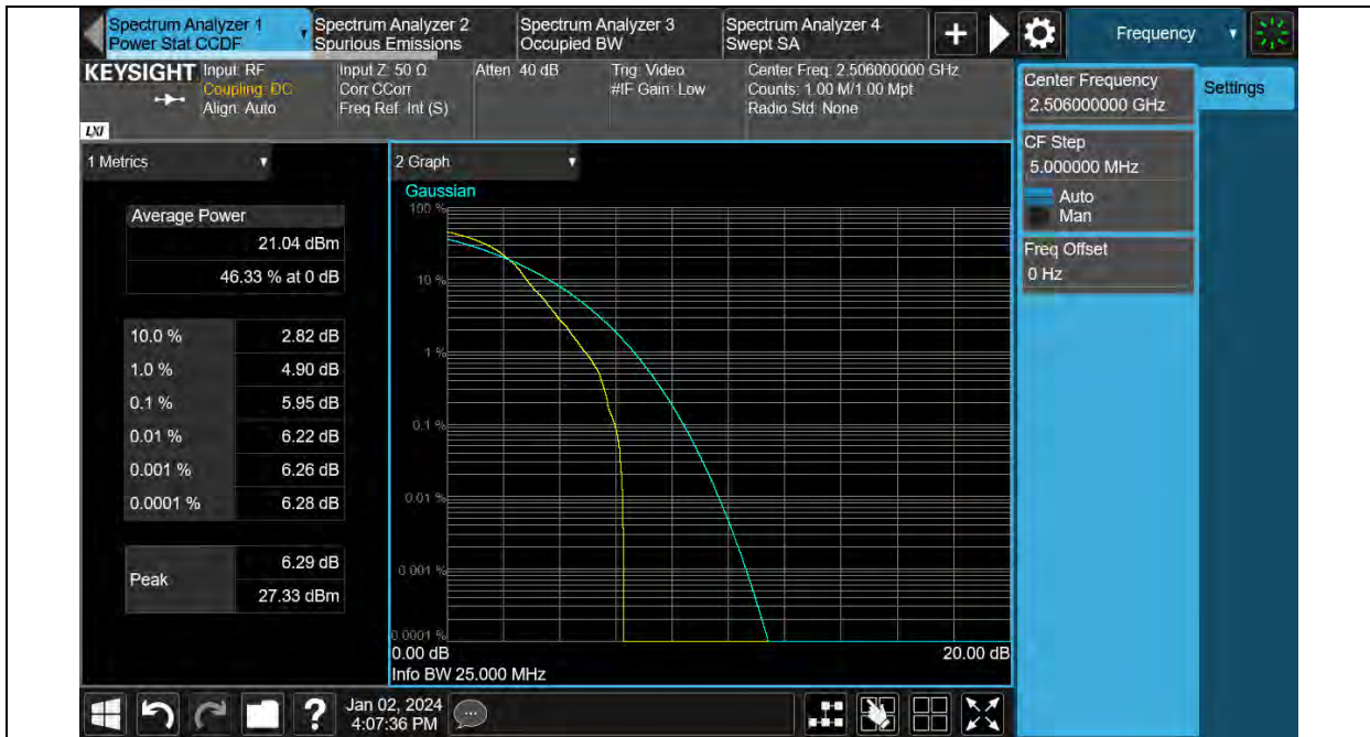
Band41-20MHz-64QAM-39750-100RB#0
