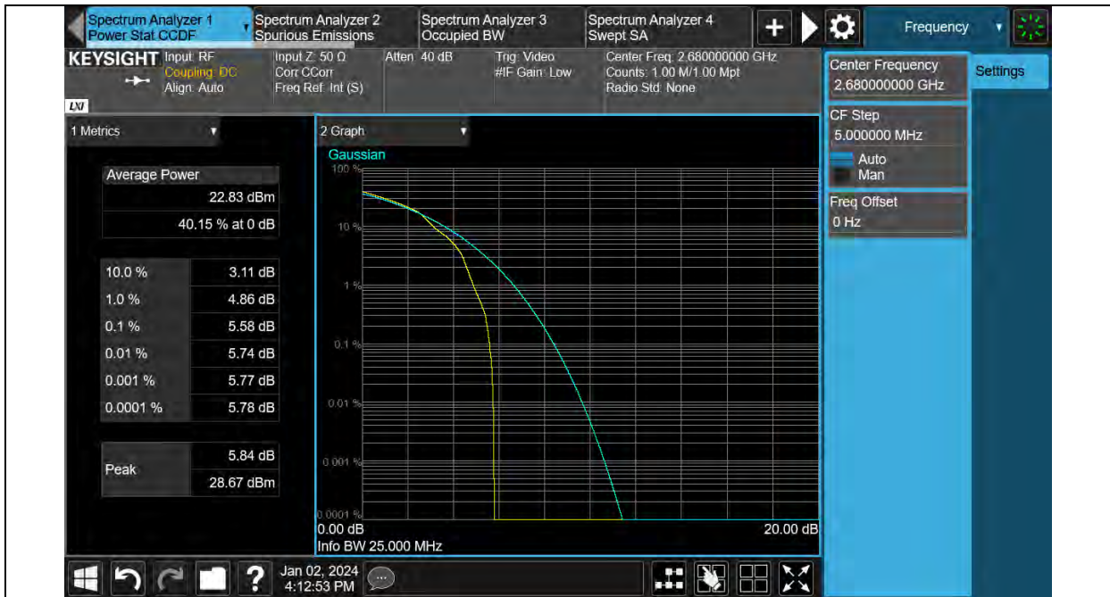
Band41-20MHz-16QAM-41490-100RB#0
