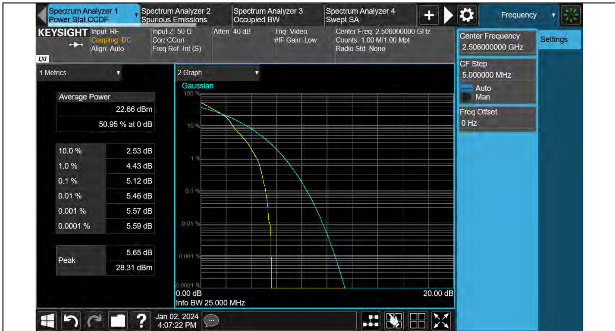
Band41-20MHz-16QAM-39750-100RB#0
