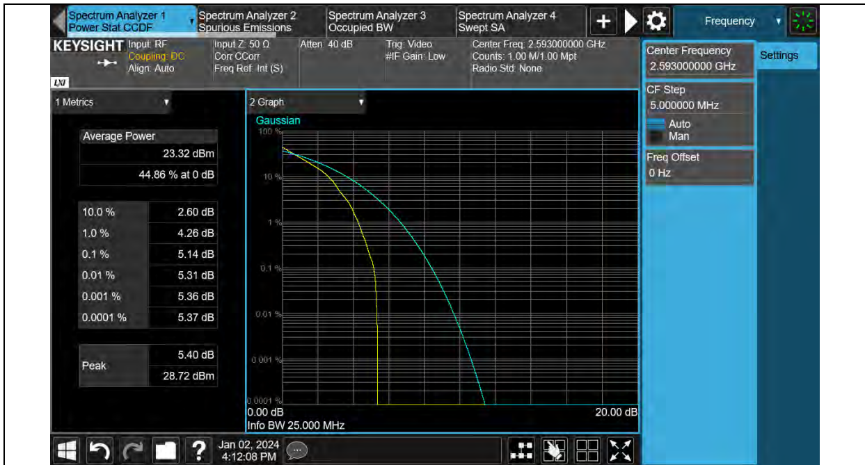
Band41-20MHz-QPSK-40620-100RB#0
