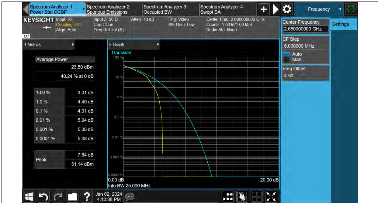
Band41-20MHz-QPSK-41490-100RB#0
