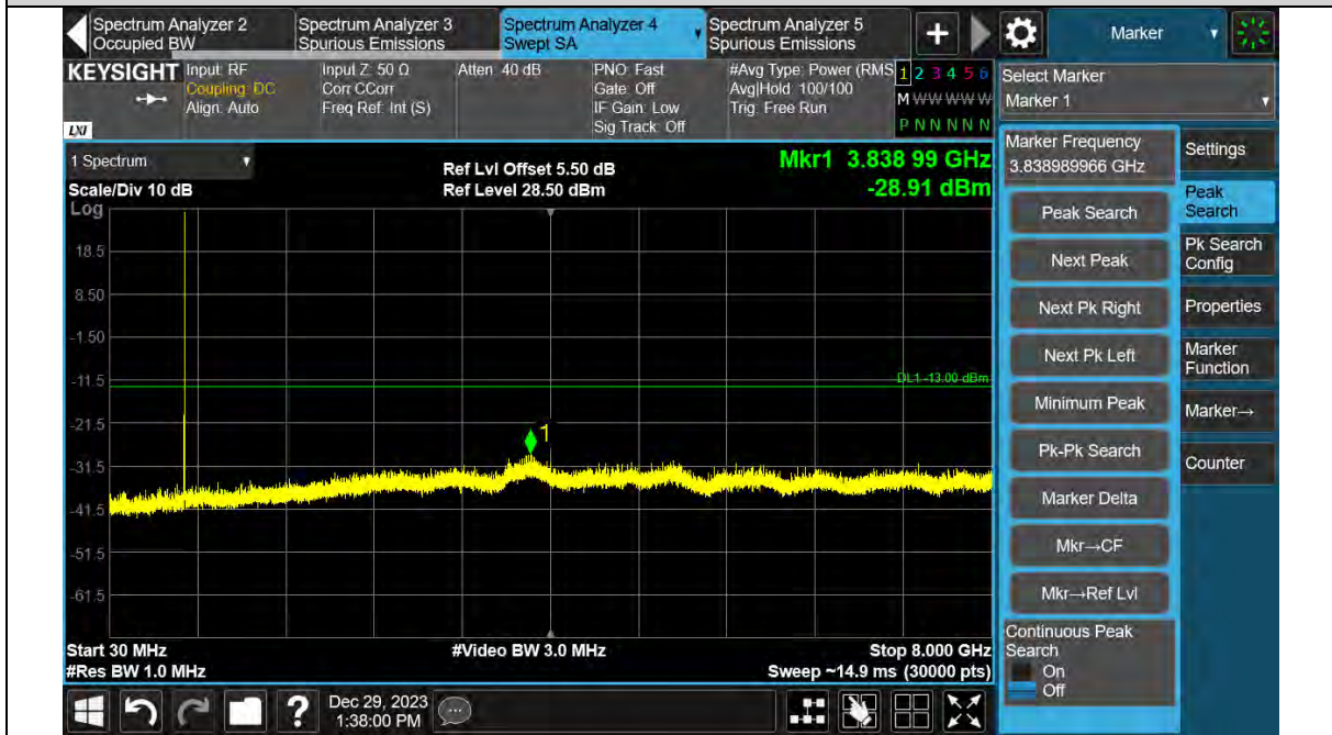
Band12-3MHz-16QAM-23165-1RB#0-30~8000MHz
