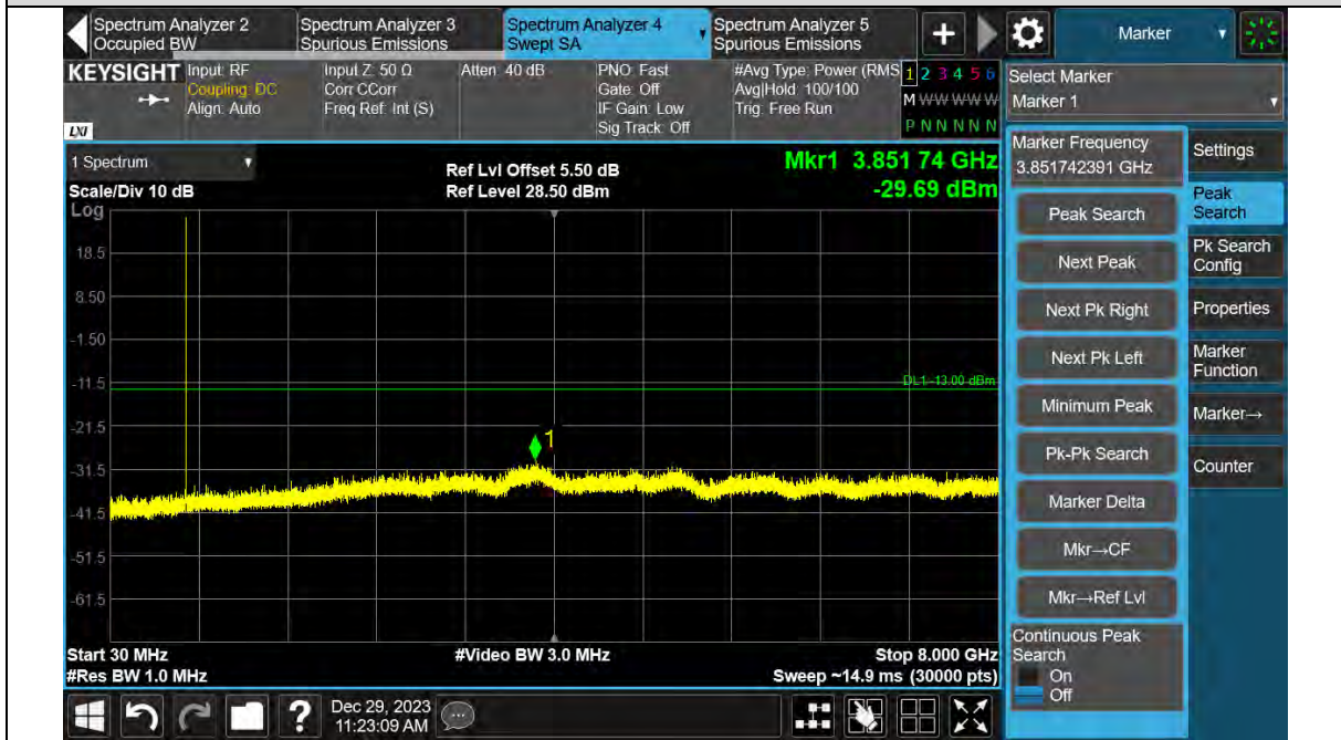
Band12-1.4MHz-64QAM-23173-1RB#0-30~8000MHz
