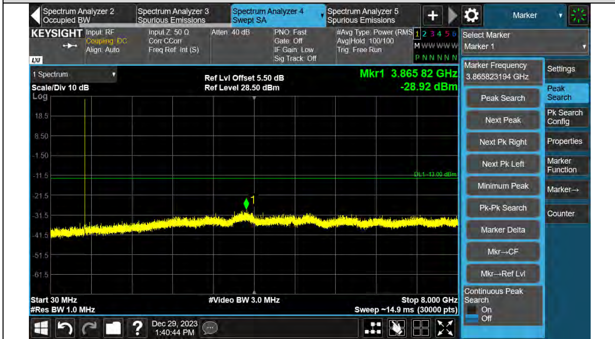
Band12-3MHz-64QAM-23095-1RB#0-30~8000MHz
