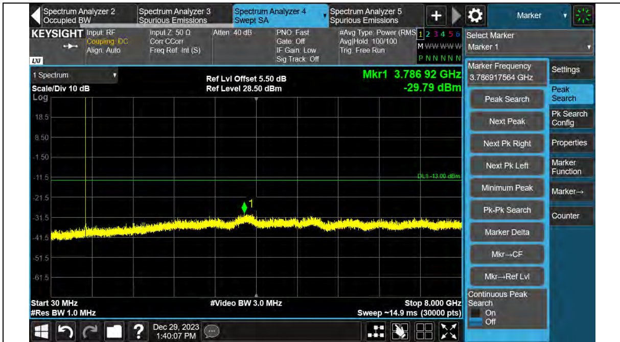
Band12-3MHz-16QAM-23095-1RB#0-30~8000MHz
