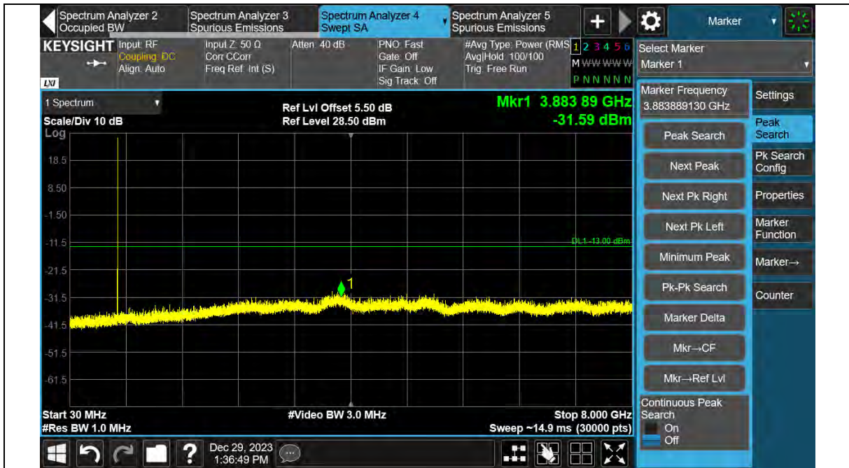
Band 12-3MHz-64QAM-23165-1RB#0-30~8000MHz
