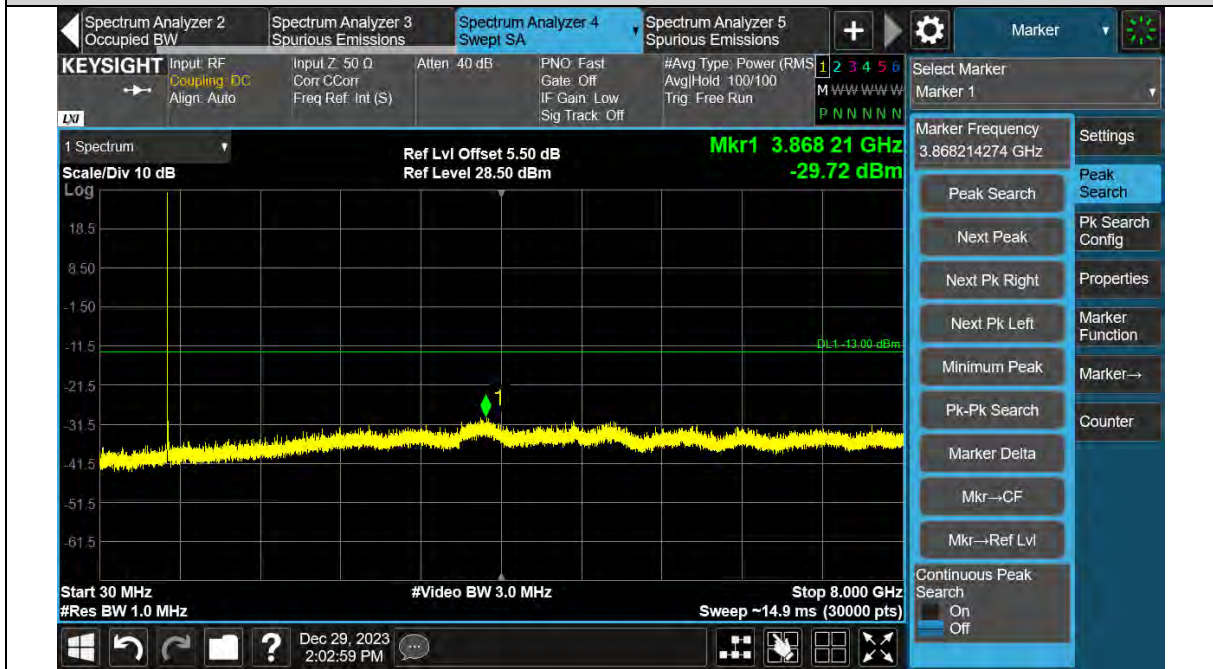
Band12-5MHz-16QAM-23095-1RB#0-30~8000MHz
