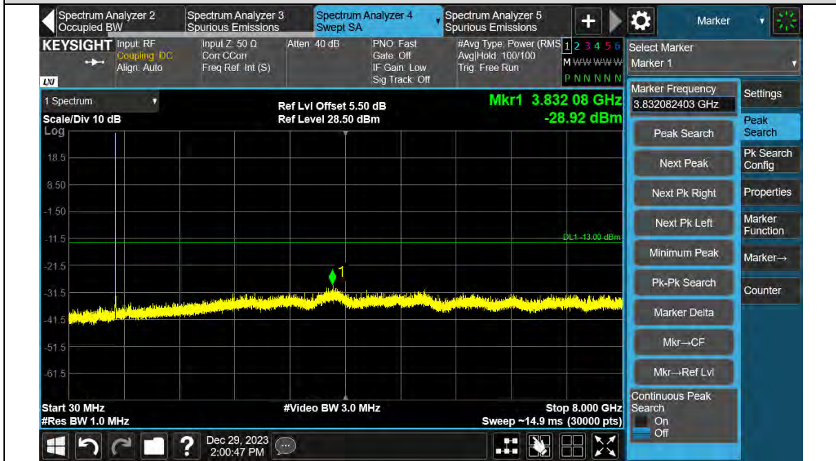
Band 12-5MHz-QPSK-23035-1RB#0-30~8000MHz
