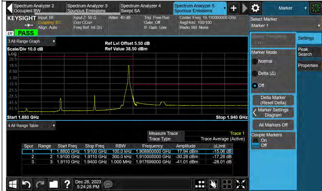
Band2-20MHz-64QAM-19100-100RB#0
