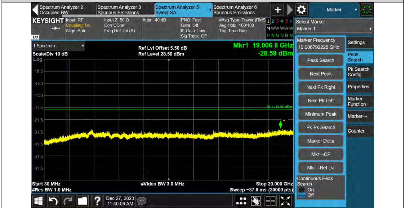
Band2-3MHz-16QAM-18900-1RB#0-30~20000MHz
