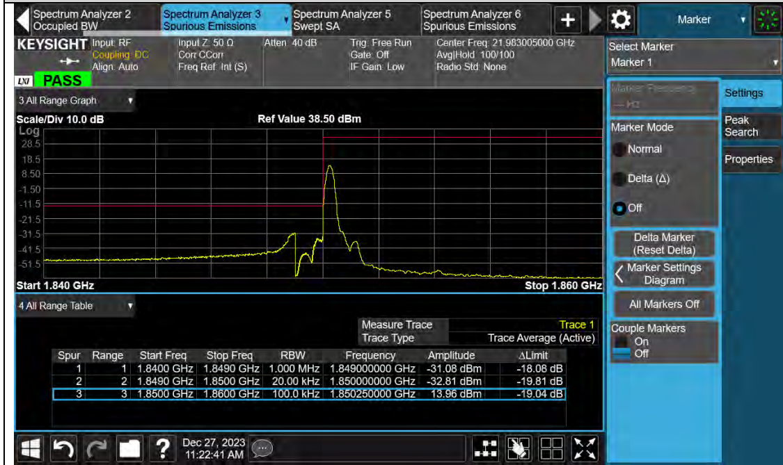
Band2-1.4MHz-64QAM-18607-6RB#0
