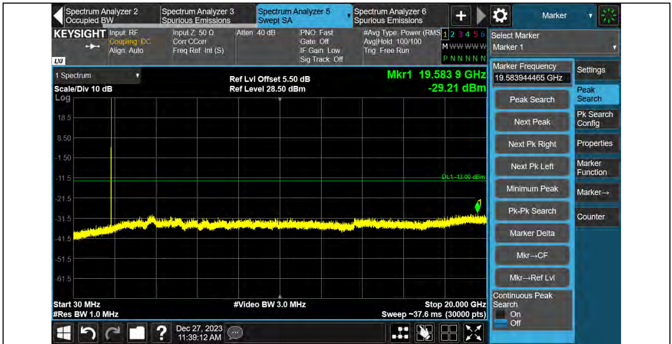
Band2-3MHz-QPSK-18900-1RB#0-30~20000MHz
