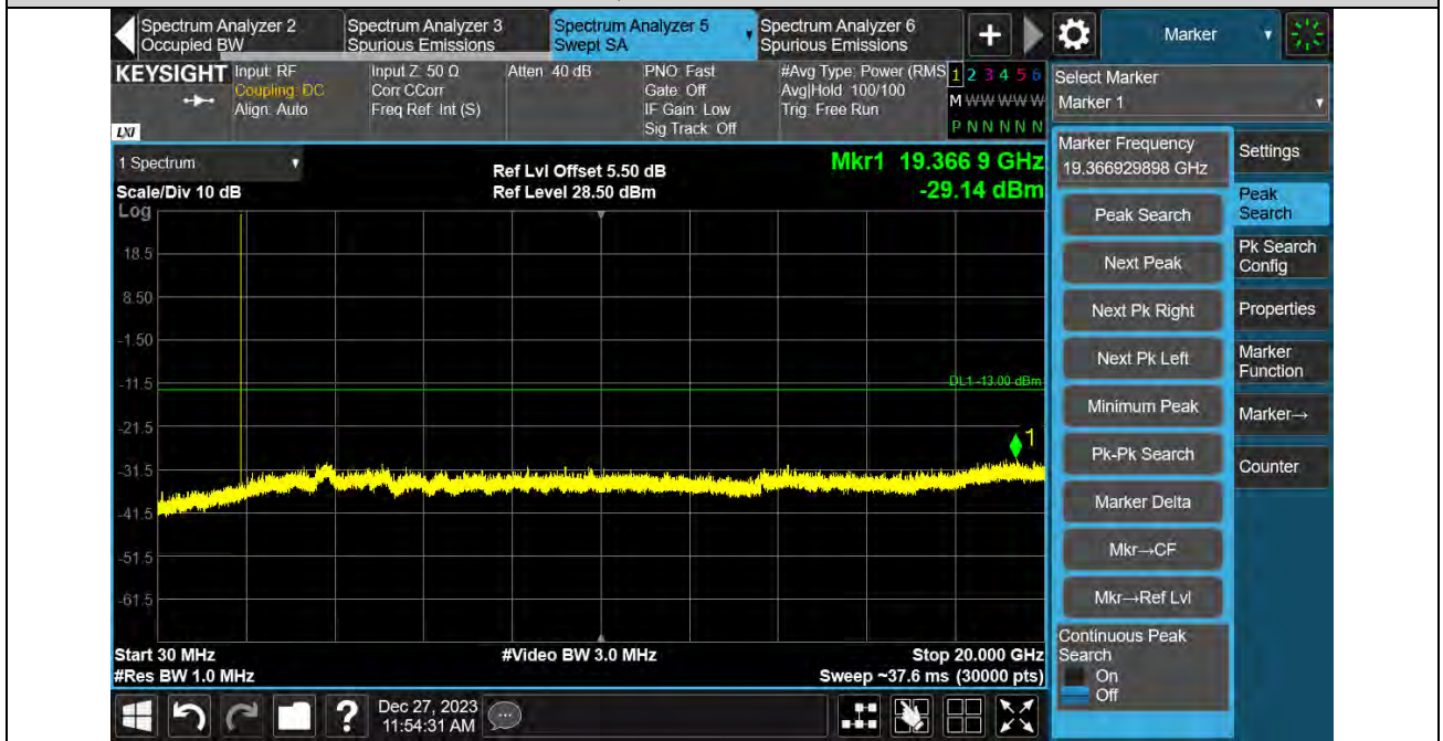
Band2-5MHz-QPSK-18625-1RB#0-30~20000MHz
