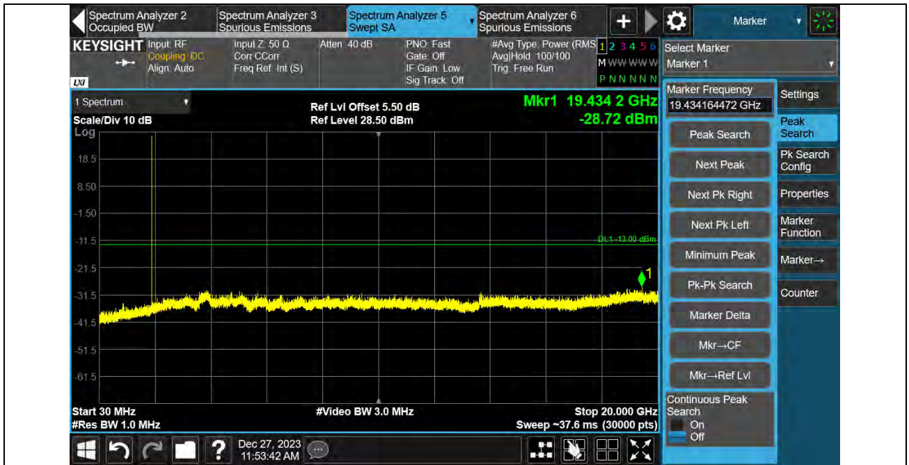
Band2-3MHz-16QAM-18615-1RB#0-30~20000MHz
