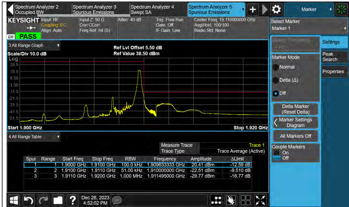
Band2-5MHz-QPSK-19175-25RB#0
