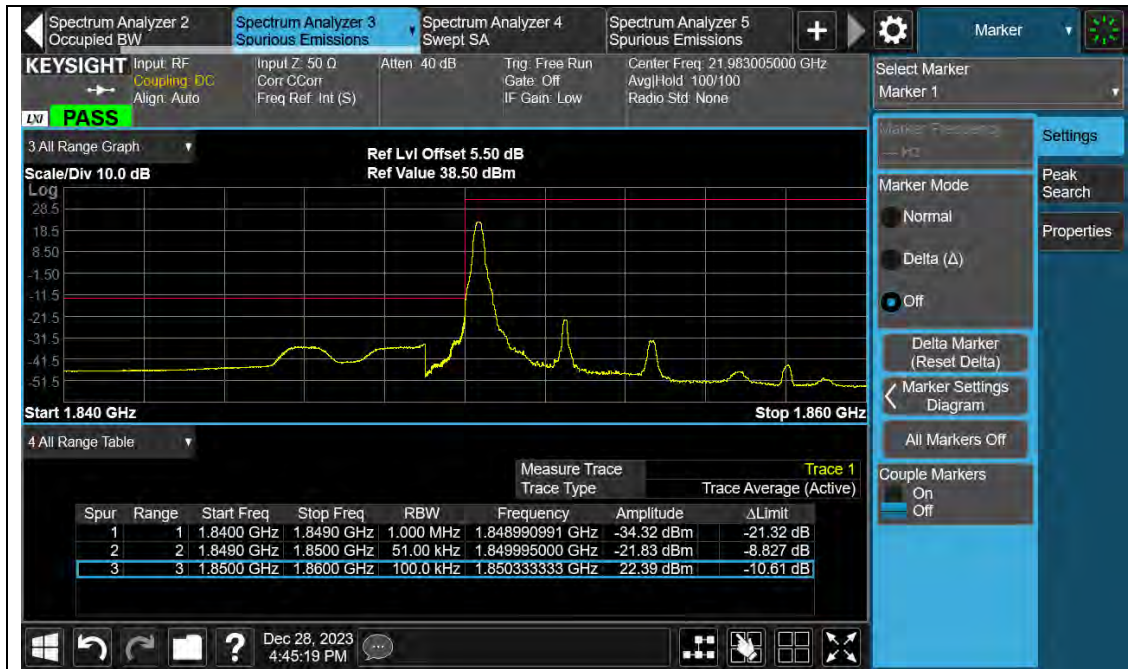
Band2-5MHz-16QAM-18625-25RB#0
