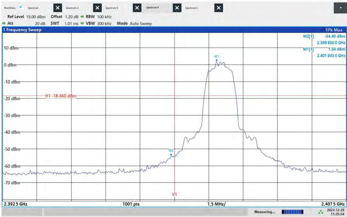
2DH5_Ant1_Low_2402
