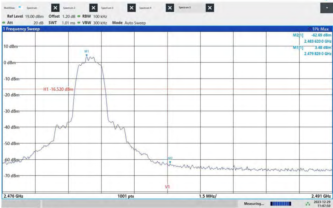
2DH5_Ant1_High_2480
