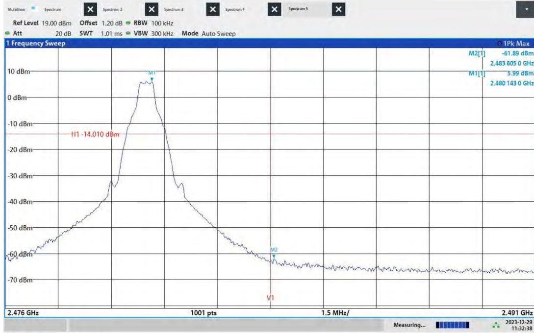
DH5_Ant1_High_2480
