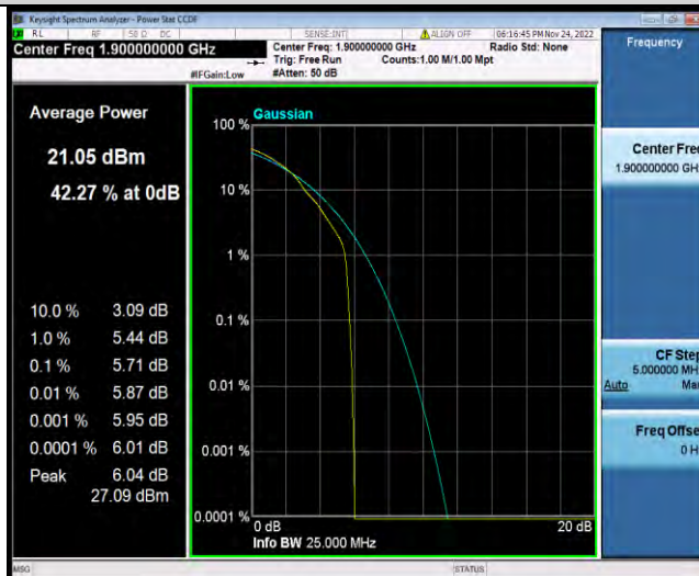
Band2-20MHz-64QAM-19100-100RB#0
