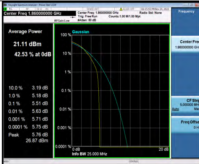
Band2-20MHz-64QAM-18700-100RB#0
