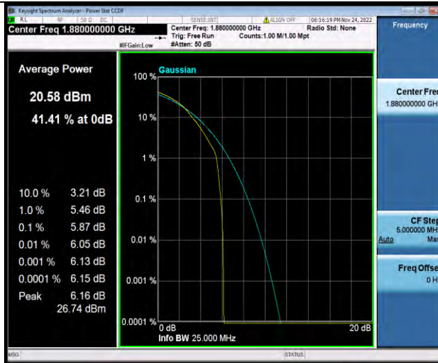
Band2-20MHz-64QAM-18900-100RB#0
