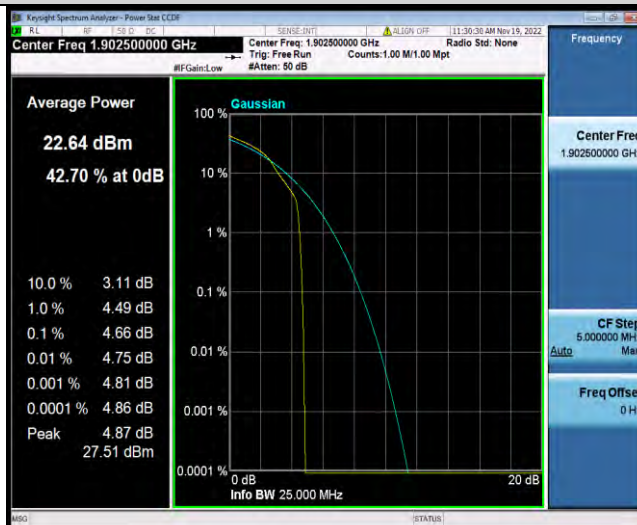
Band2-15MHz-16QAM-19125-75RB#0
