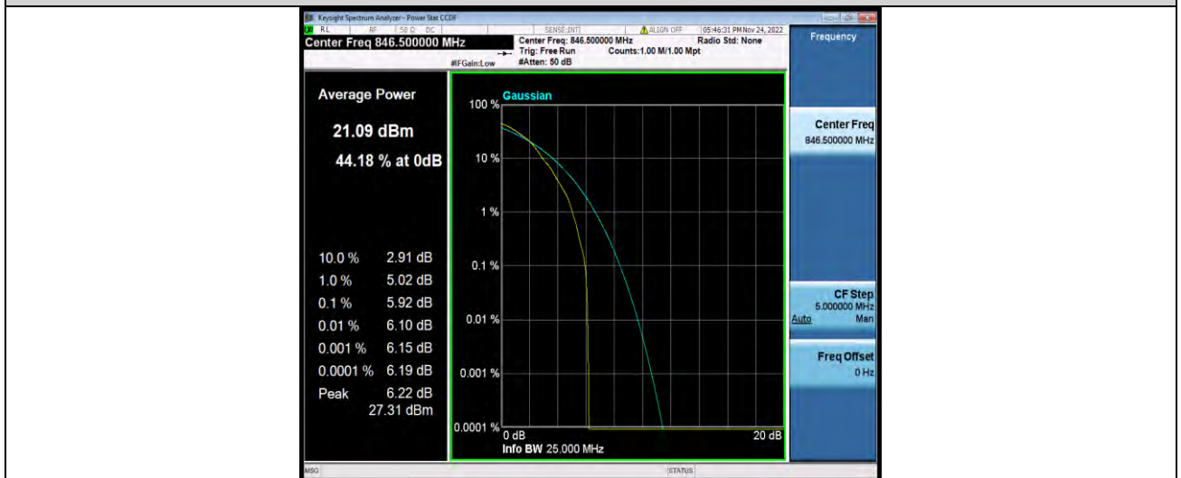
Band26-5MHz-64QAM-27015-25RB#0
