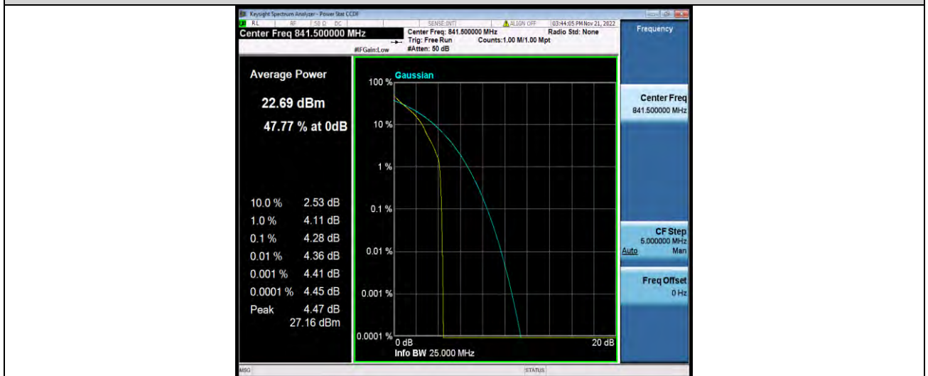
Band26-15MHz-QPSK-26965-75RB#0
