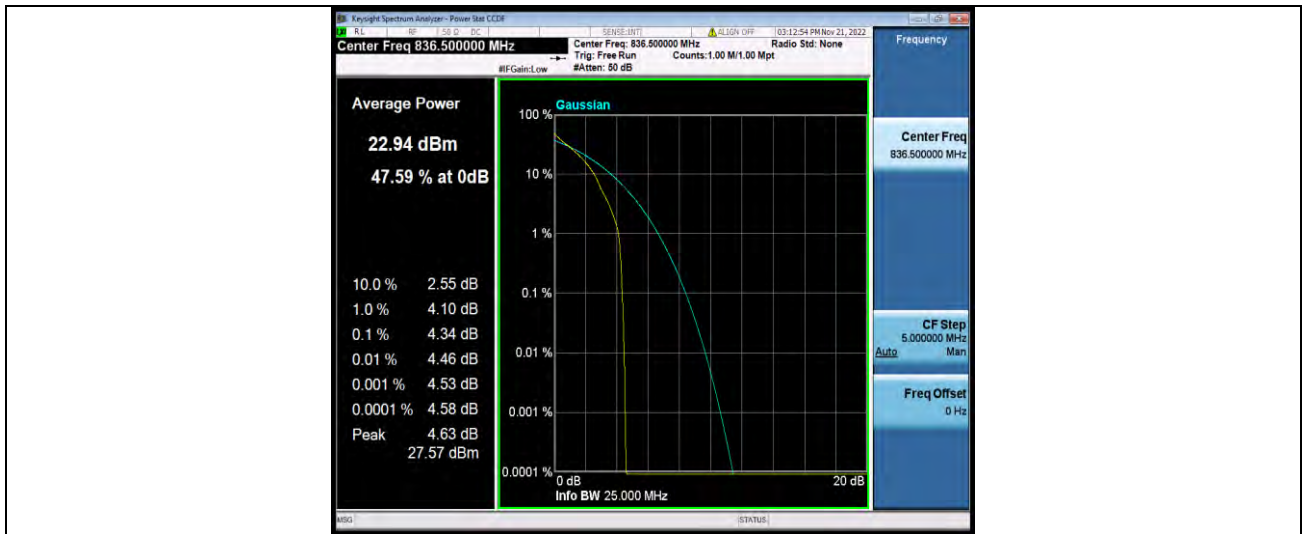
Band26-5MHz-QPSK-26915-25RB#0
