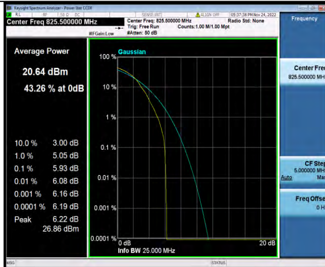
Band26-3MHz-64QAM-26805-15RB#0
