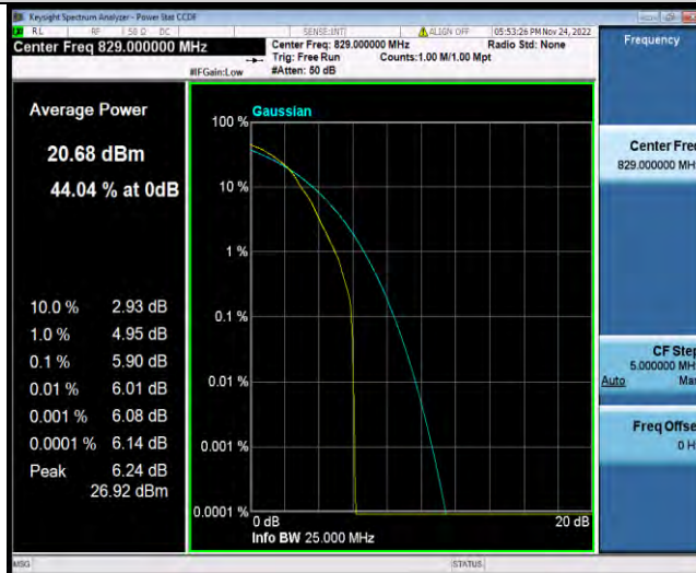
Band26-10MHz-64QAM-26840-50RB#0
