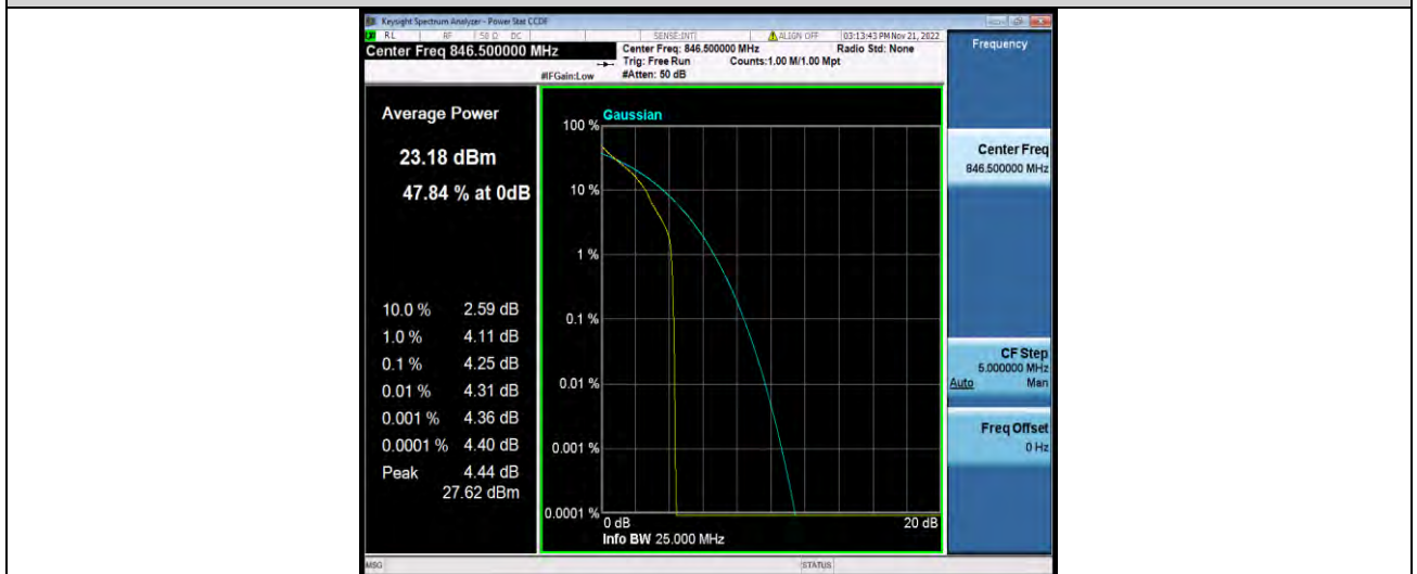
Band26-5MHz-QPSK-27015-25RB#0
