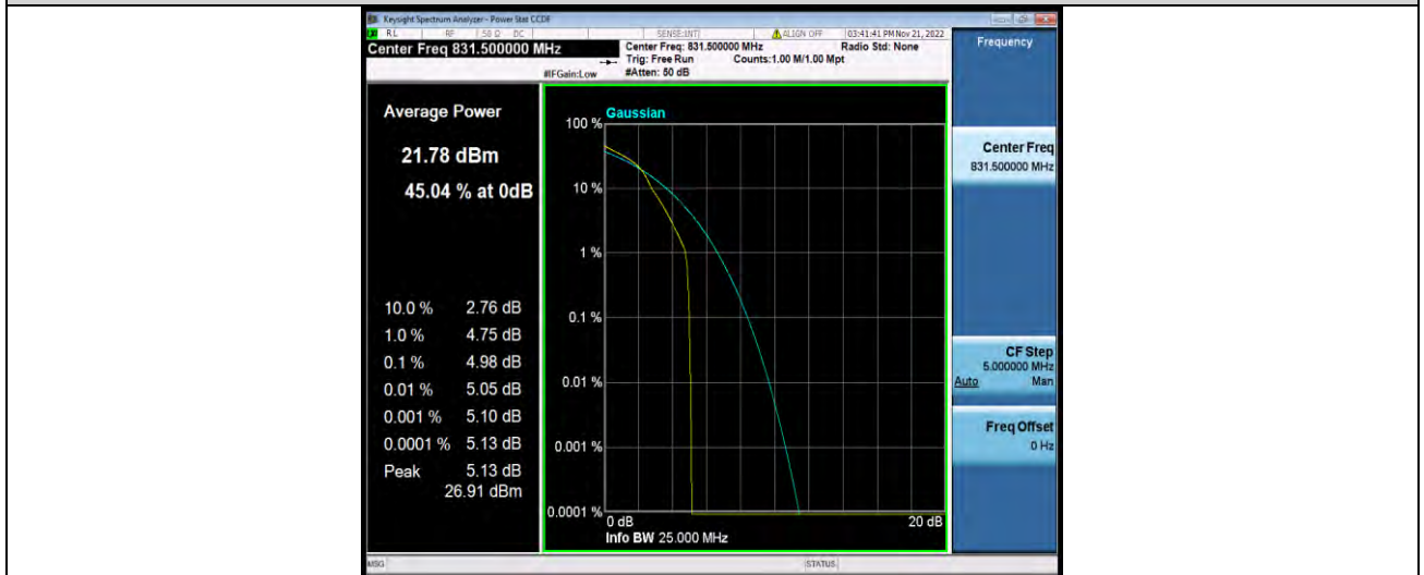
Band26-15MHz-16QAM-26865-75RB#0
