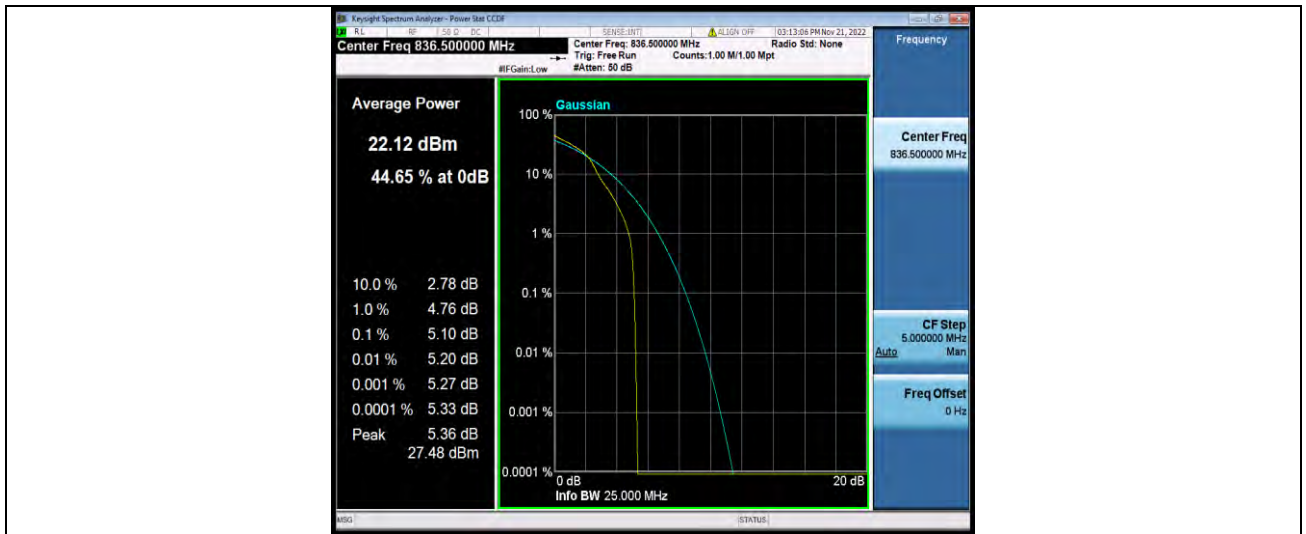
Band26-5MHz-16QAM-26915-25RB#0
