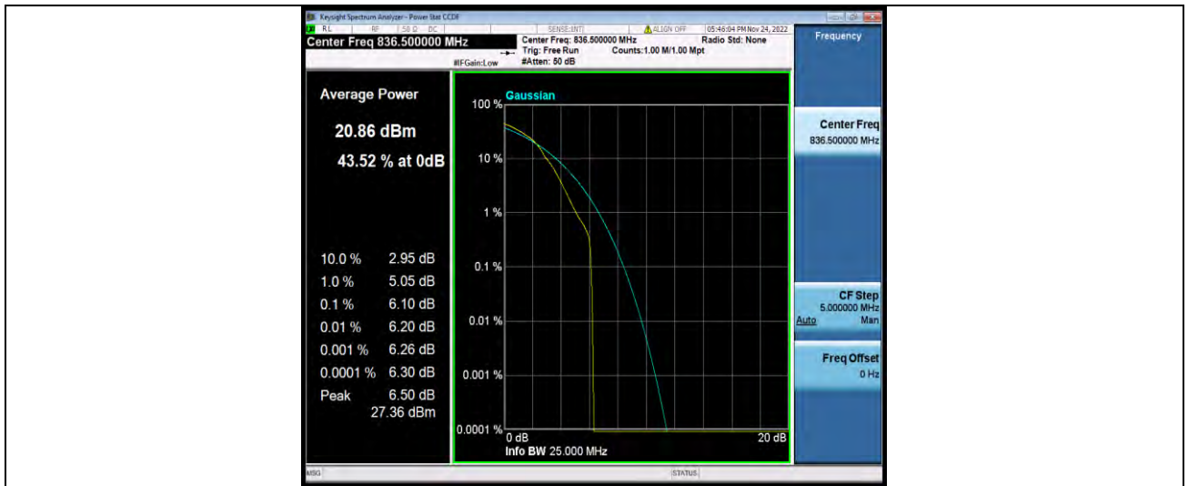
Band26-5MHz-64QAM-26915-25RB#0
