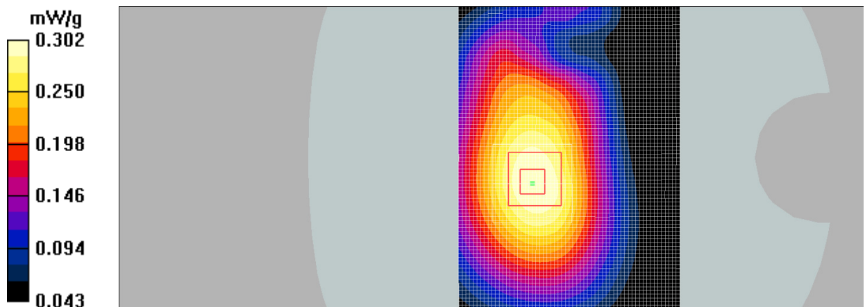
Fig.6 WCDMA 850 CH4132
