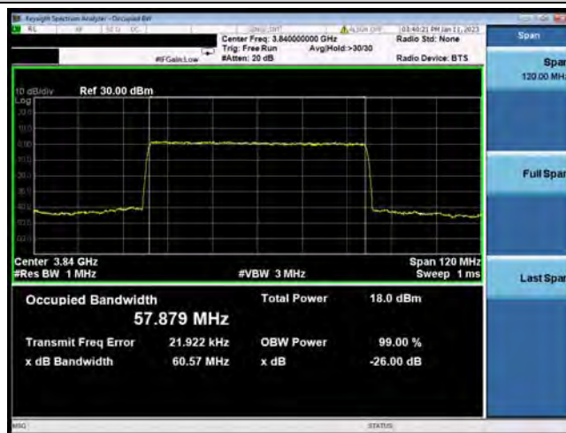
N77-60MHz-BPSK-656000-162RB#0
