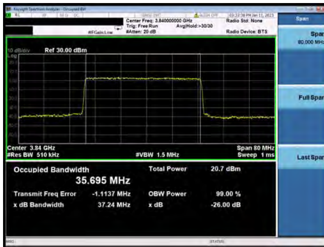
N77-40MHz-256QAM-656000-100RB#0
