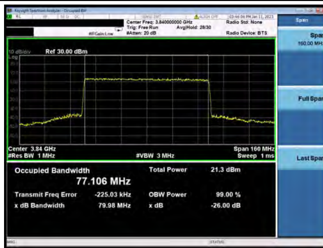
N77-80MHz-16QAM-656000-216RB#0
