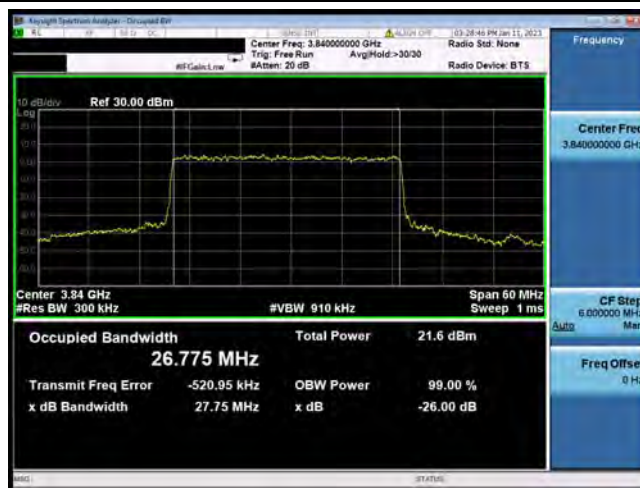
N77-30MHz-16QAM-656000-75RB#0
