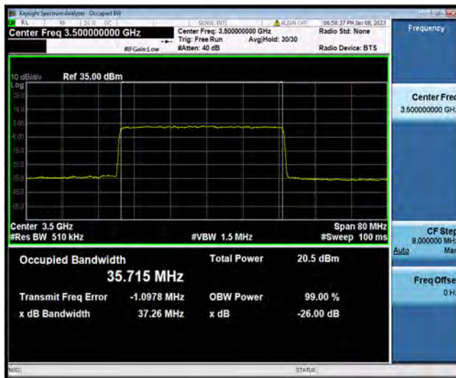
N78-40MHz-256QAM-633334-100RB#0
