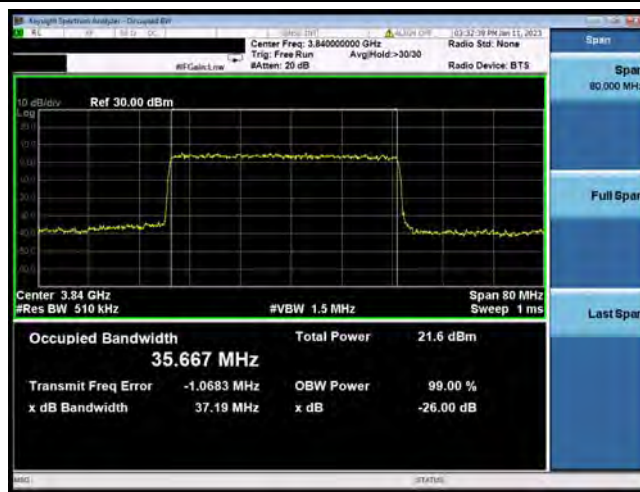
N77-40MHz-16QAM-656000-100RB#0
