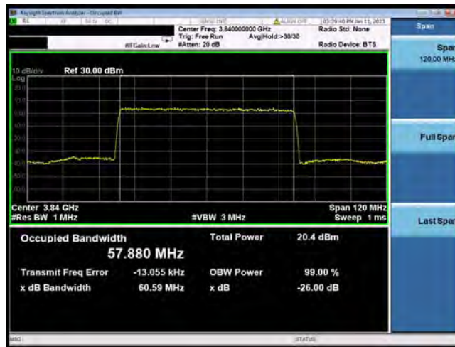
N77-60MHz-64QAM-656000-162RB#0
