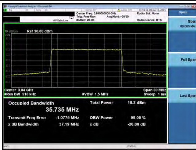
N77-40MHz-BPSK-656000-100RB#0
