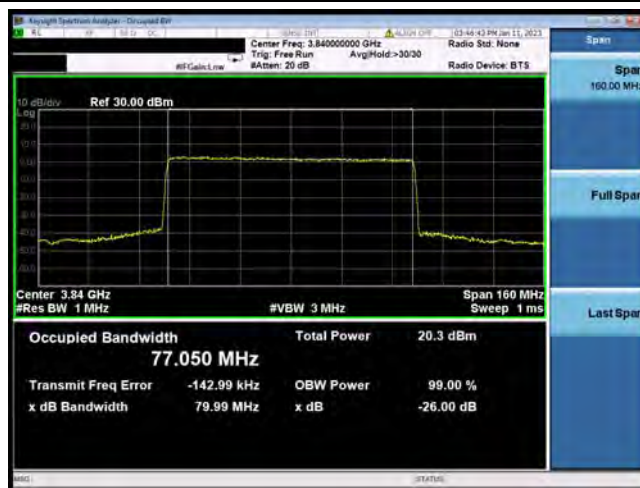
N77-80MHz-64QAM-656000-216RB#0
