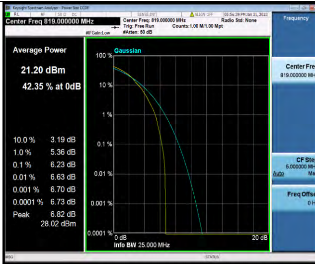
Band26-3MHz-64QAM-26740-15RB#0
