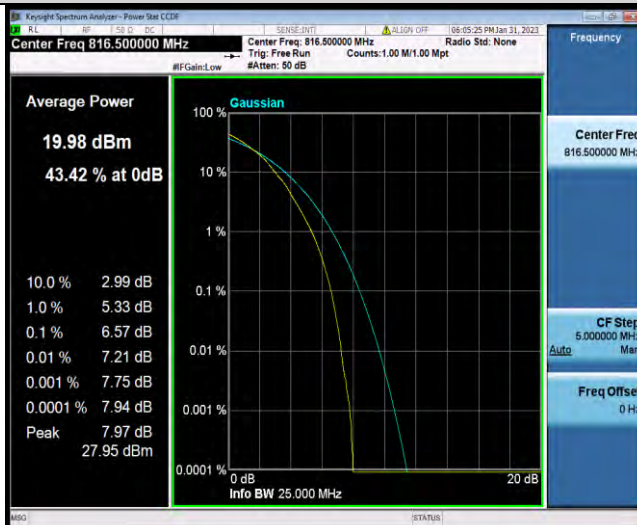
Band26-5MHz-64QAM-26740-1RB#0
