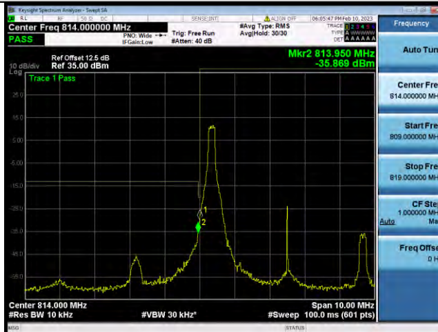
Band26-5MHz-16QAM-26715-25RB#0
