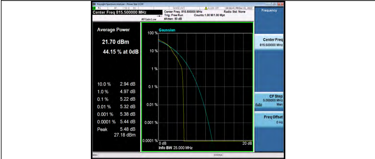
Band26-3MHz-16QAM-26705-15RB#0
