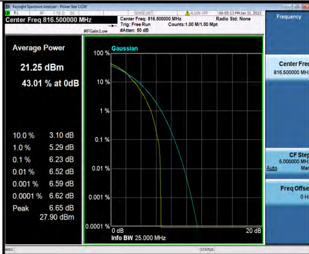
Band26-5MHz-64QAM-26715-25RB#0
