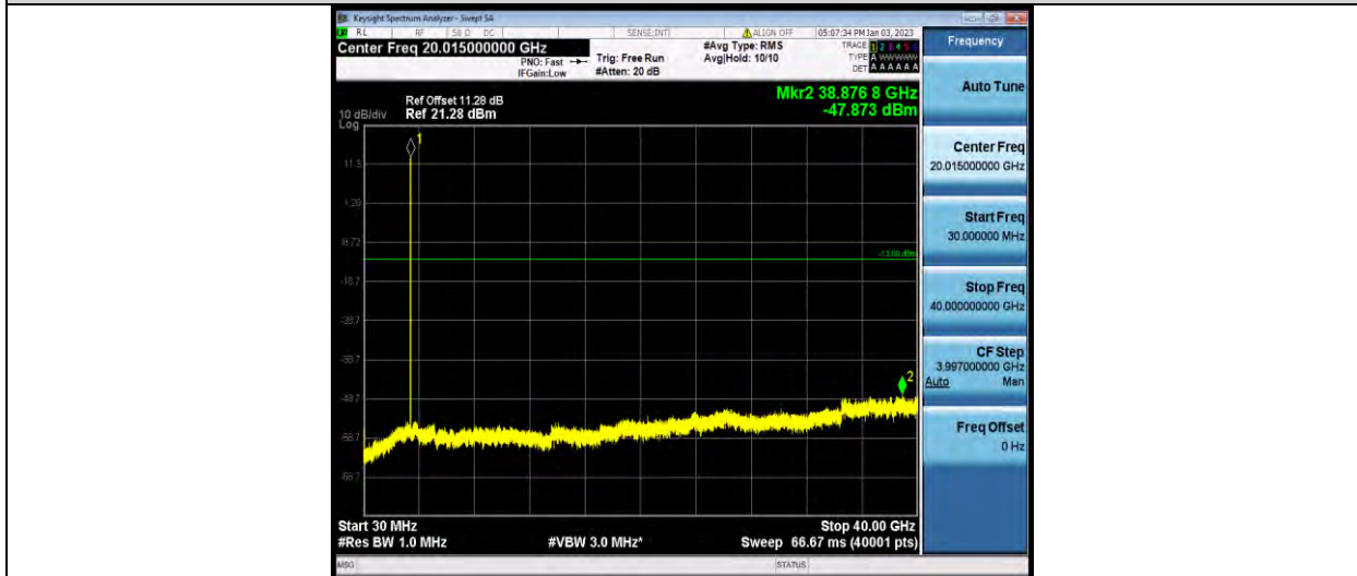
42-42-20MHz-20MHz-16QAM-16QAM-42491-42689-1RB#99-1RB#0-30~40000MHz
