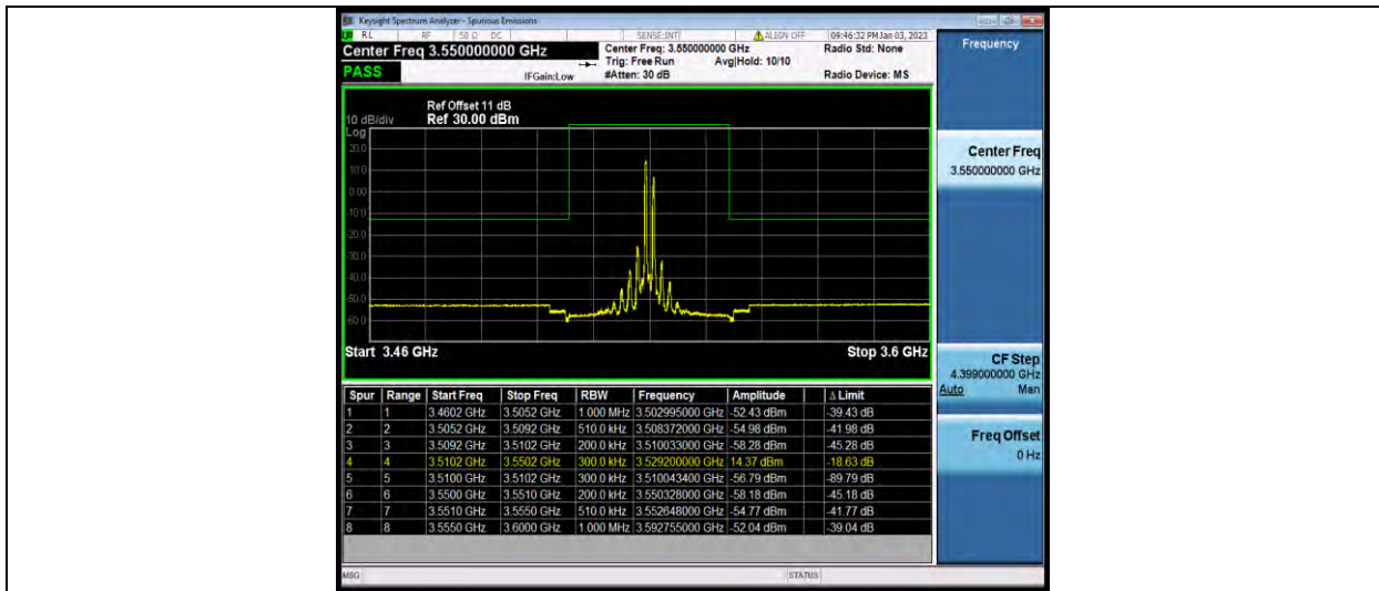
42-42-20MHz-20MHz-16QAM-16QAM-41690-41888-100RB#0-100RB#0
