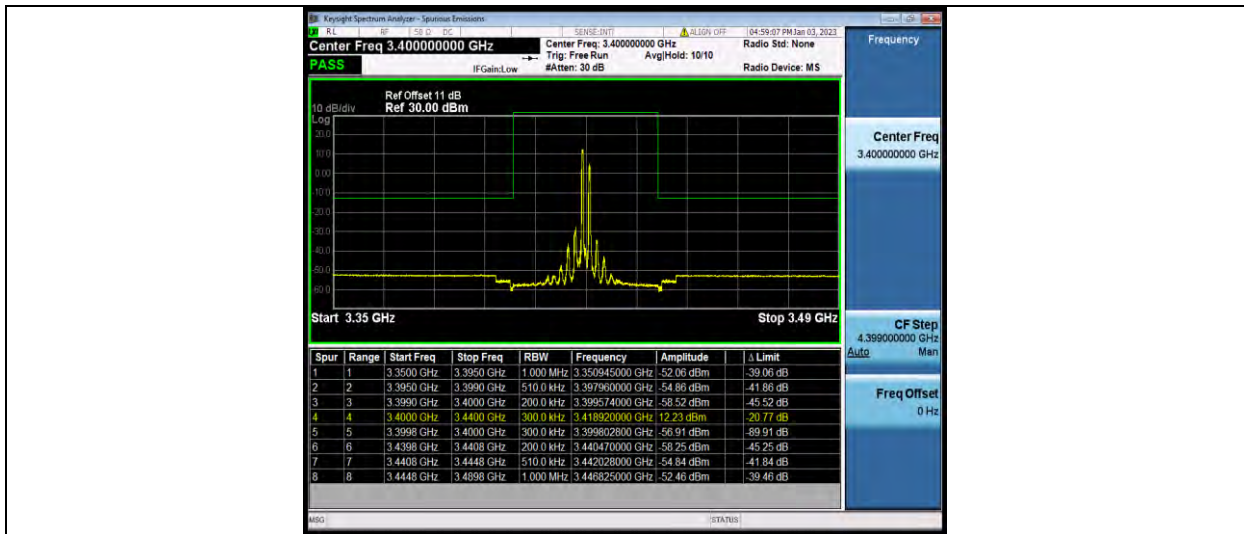
42-42-20MHz-20MHz-64QAM-64QAM-42792-42990-100RB#0-100RB#0
