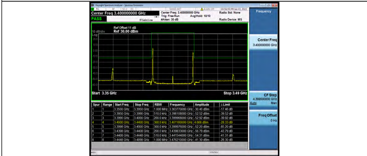
42-42-20MHz-20MHz-16QAM-16QAM-41690-41888-1RB#99-1RB#0
