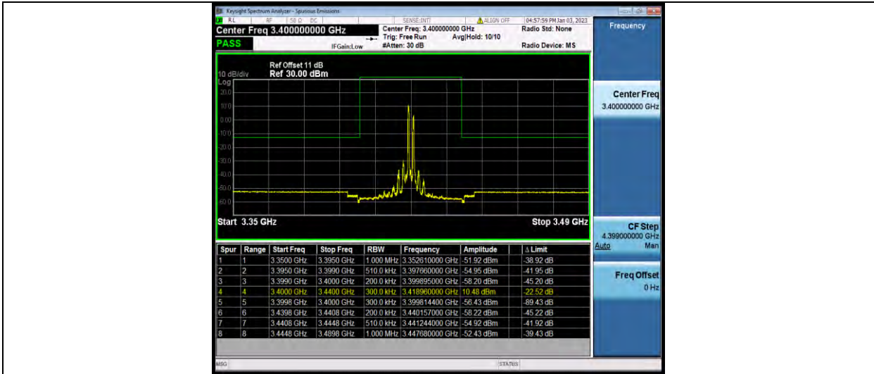
42-42-20MHz-20MHz-QPSK-QPSK-42792-42990-100RB#0-100RB#0
