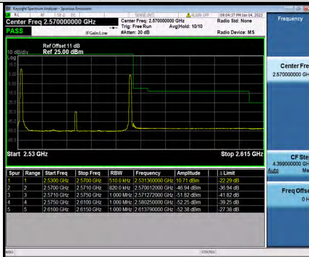
7-7-20MHz-20MHz-QPSK-QPSK-21152-21350-1RB#99-1RB#0
