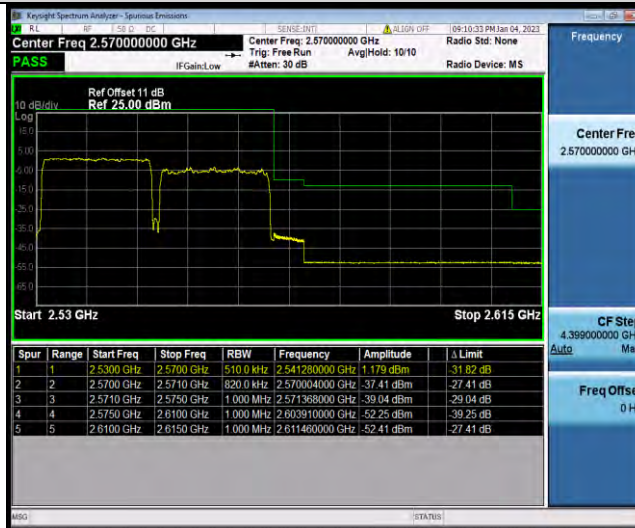
7-7-20MHz-20MHz-QPSK-QPSK-21152-21350-1RB#0-1RB#99
