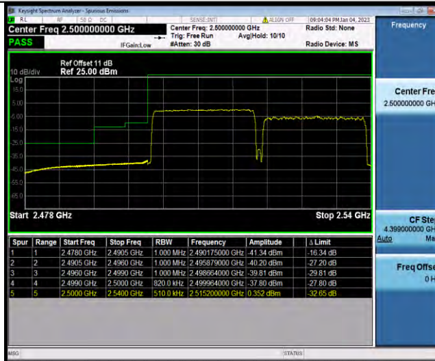
7-7-20MHz-20MHz-64QAM-64QAM-20850-21048-1RB#0-1RB#99
