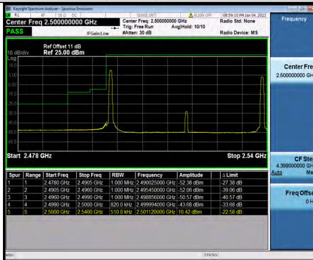
7-7-20MHz-20MHz-64QAM-64QAM-20850-21048-1RB#99-1RB#0
