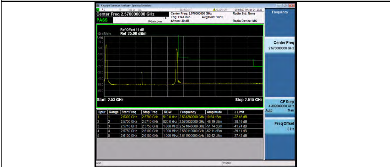
7-7-20MHz-20MHz-16QAM-16QAM-21152-21350-1RB#99-1RB#0
