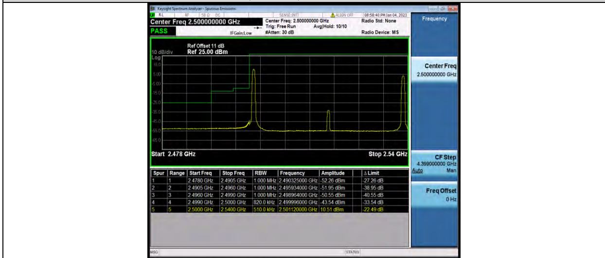
7-7-20MHz-20MHz-16QAM-16QAM-20850-21048-1RB#99-1RB#0
