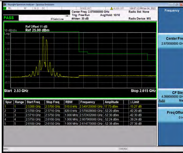
7-7-20MHz-20MHz-64QAM-64QAM-20850-21048-100RB#0-100RB#0
