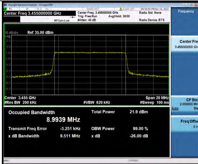
Band42-10MHz-QPSK-42590-50RB#0
