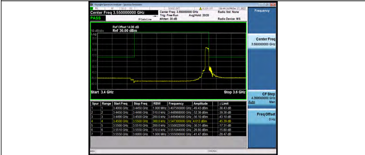
Band42-5MHz-16QAM-42115-1RB#0
