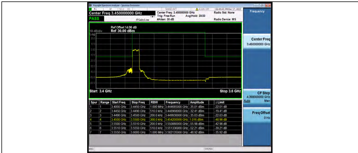
Band42-10MHz-16QAM-43040-1RB#49
