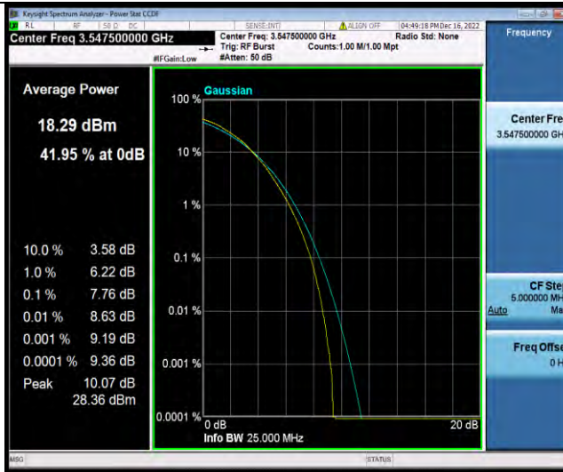
Band42-10MHz-QPSK-42140-1RB#0
