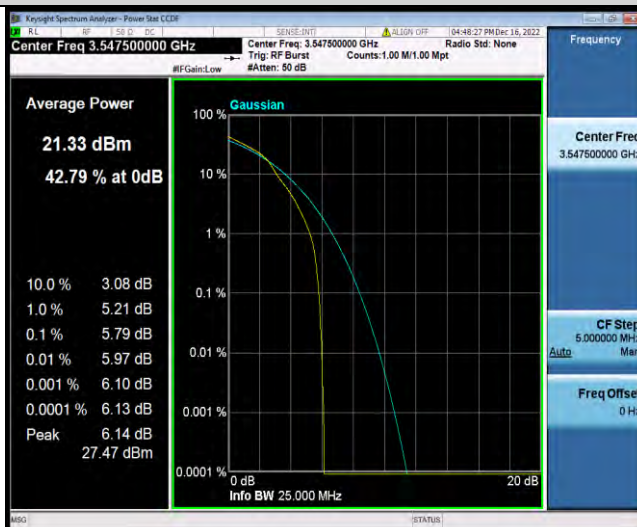
Band42-5MHz-16QAM-43065-25RB#0
