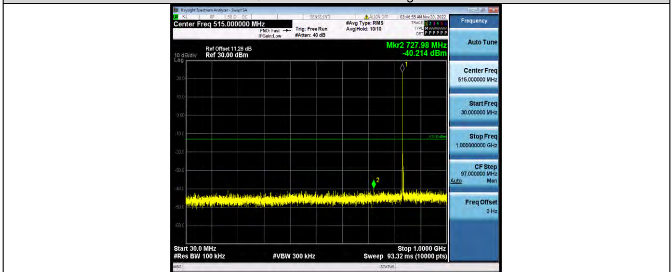
Band26-5MHz-QPSK-26915-1RB#0-Range2:1000~10000MHz
