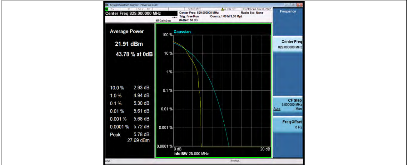
Band26-10MHz-16QAM-26840-50RB#0
