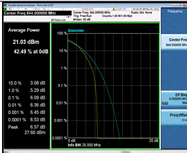
Band26-10MHz-64QAM-26990-50RB#0
