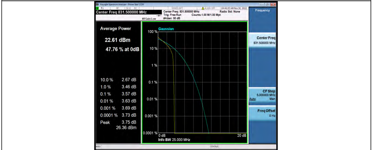
Band26-15MHz-QPSK-26865-75RB#0
