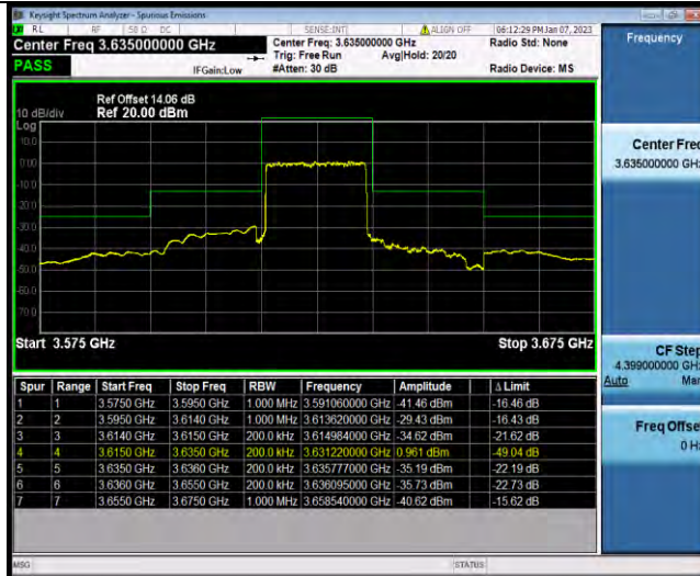
N48-20MHz-QPSK-646000-1RB#0
