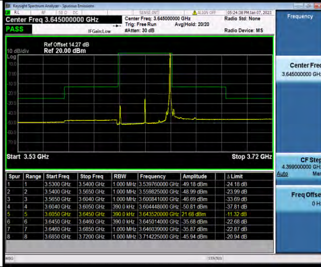
N48-40MHz-QPSK-641666-100RB#0
