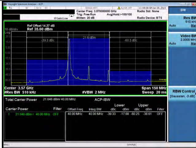
N48-40MHz-QPSK-638000-1RB#104
