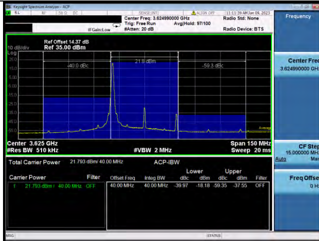
N48-40MHz-QPSK-641666-1RB#104
