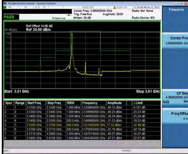
N48-20MHz-QPSK-637334-1RB#50
