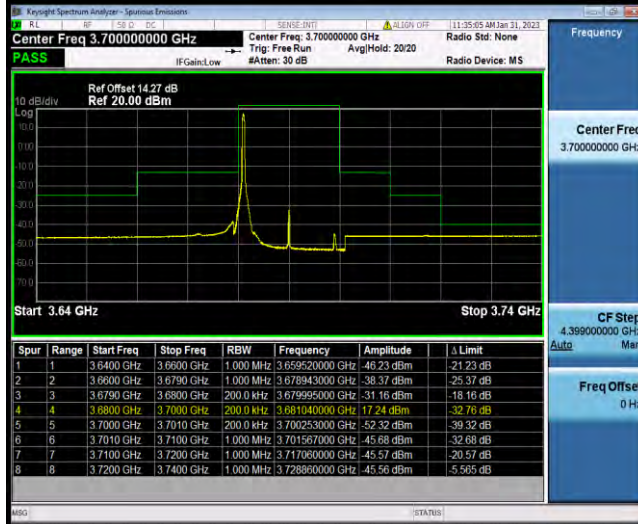
N48-20MHz-QPSK-646000-1RB#50
