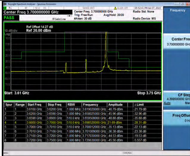
N48-40MHz-QPSK-645332-100RB#0
