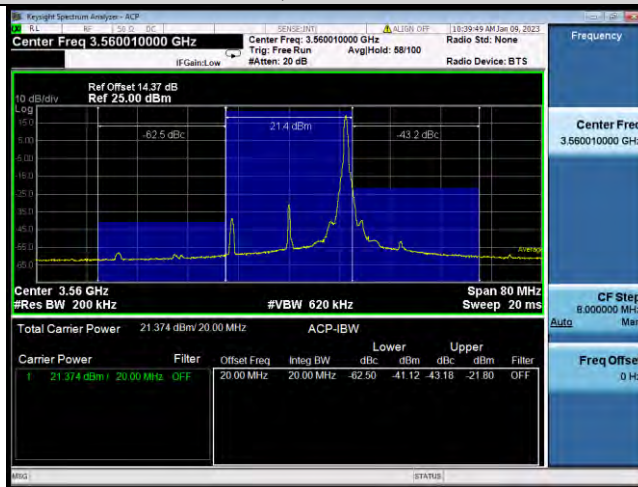
N48-20MHz-QPSK-637334-50RB#0
