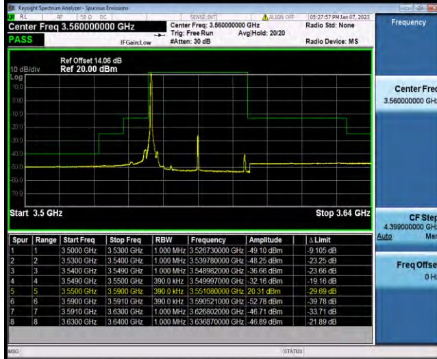
N48-40MHz-QPSK-638000-1RB#104
