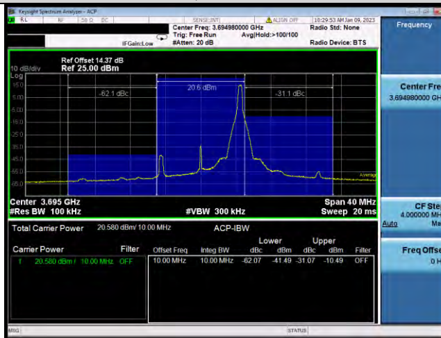
N48-10MHz-QPSK-646332-25RB#0
