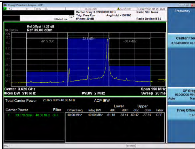
N48-40MHz-QPSK-641666-100RB#0
