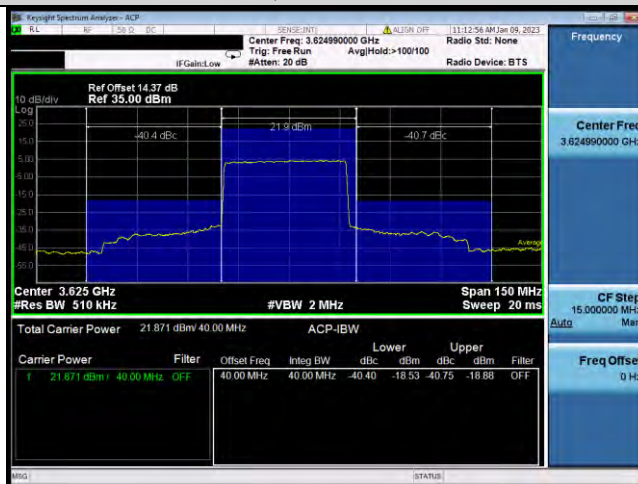
N48-40MHz-QPSK-645332-1RB#0
