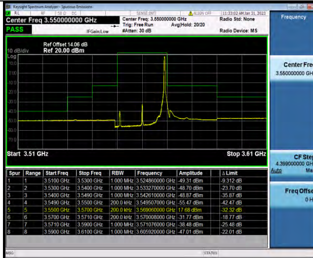
N48-20MHz-QPSK-637334-50RB#0
