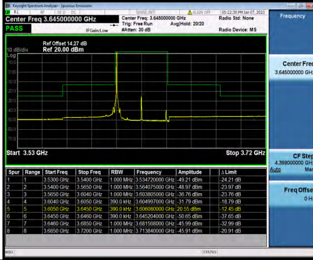
N48-40MHz-QPSK-641666-1RB#104
