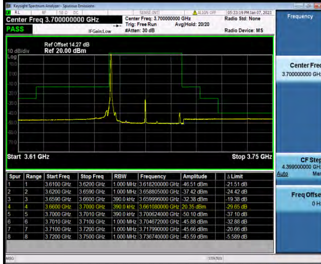
N48-40MHz-QPSK-645332-1RB#104
