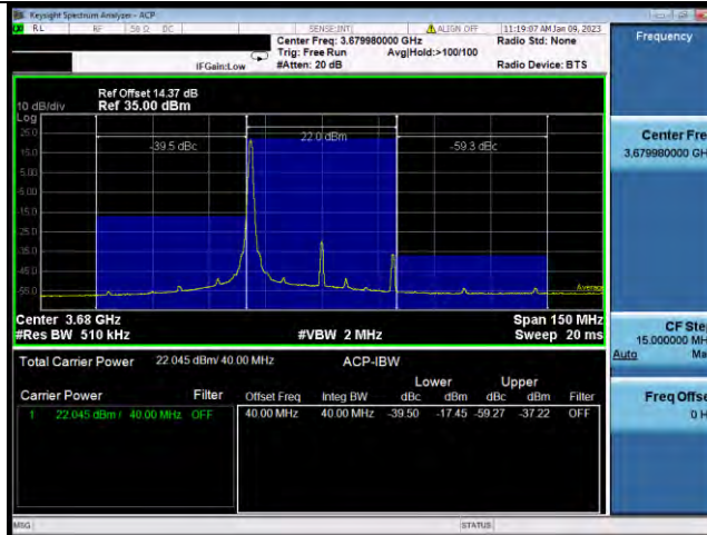
N48-40MHz-QPSK-645332-1RB#104
