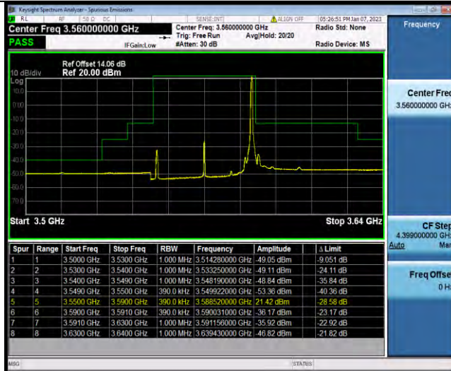
N48-40MHz-QPSK-638000-100RB#0
