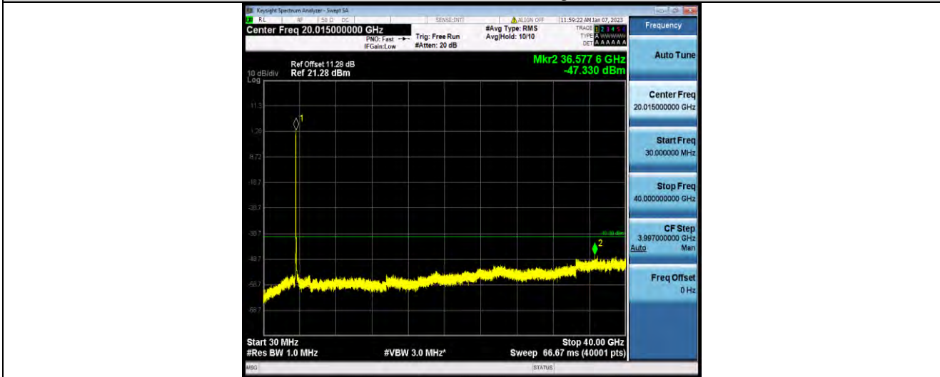
N48-40MHz-QPSK-645332-1RB#0-Range1:30~40000MHz
