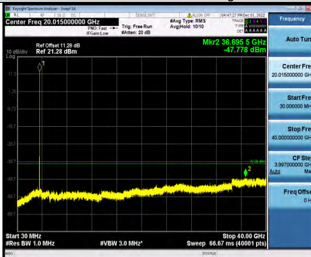
Band48-20MHz-QPSK-56640-1RB#0-Range1:30~40000MHz
