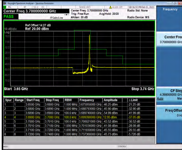
Band48-10MHz-16QAM-56690-50RB#0
