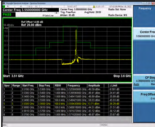
Band48-10MHz-64QAM-55290-50RB#0
