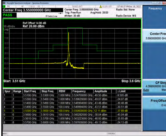
Band48-10MHz-64QAM-55290-1RB#49
