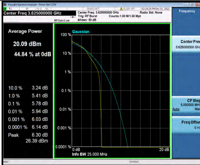
Band48-10MHz-16QAM-55990-50RB#0
