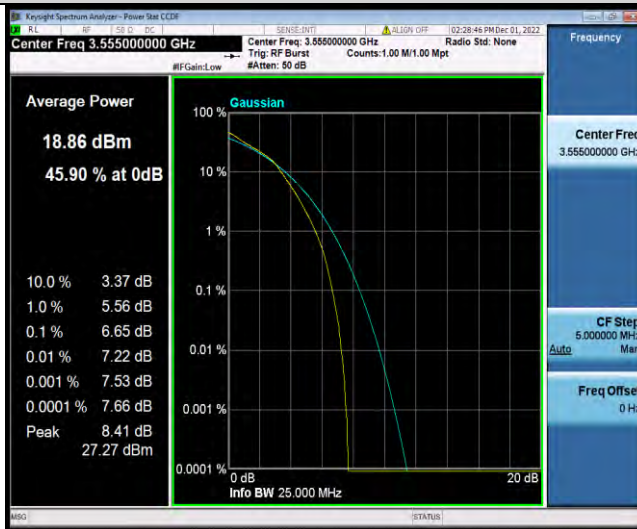
Band48-10MHz-16QAM-55990-1RB#0
