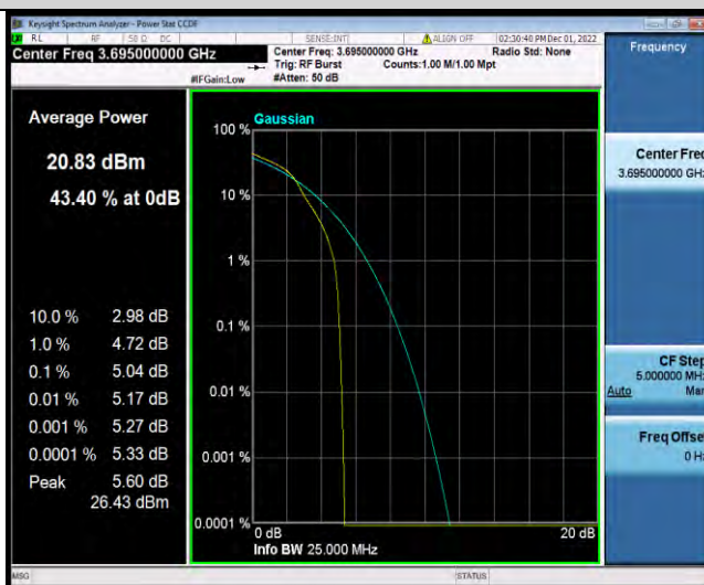
Band48-10MHz-16QAM-56690-50RB#0
