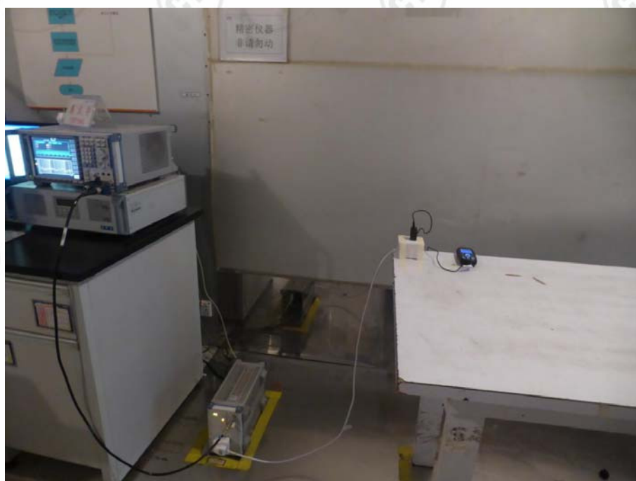
Conducted Emissions-2
