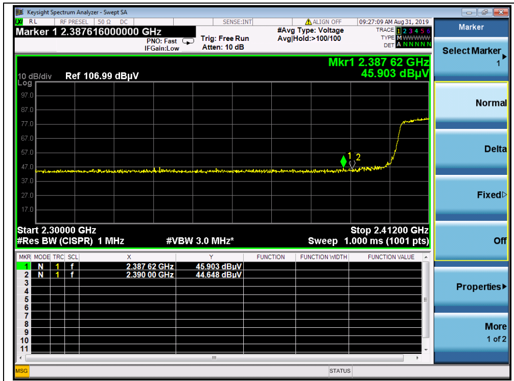
(Channel = 3 AVG, 802.11n(HT40))
