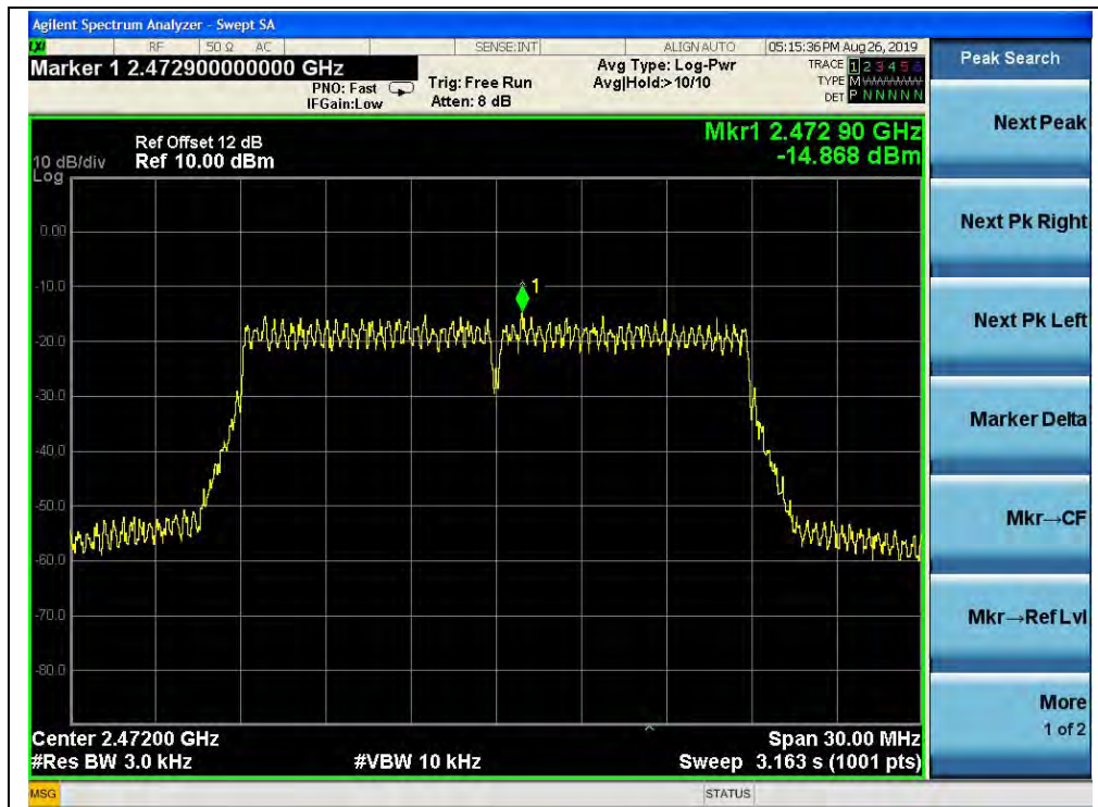
(Channel = 13, 802.11n(HT20))
