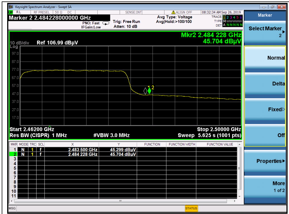
(Channel = 9 AVG, 802.11n(HT40))
