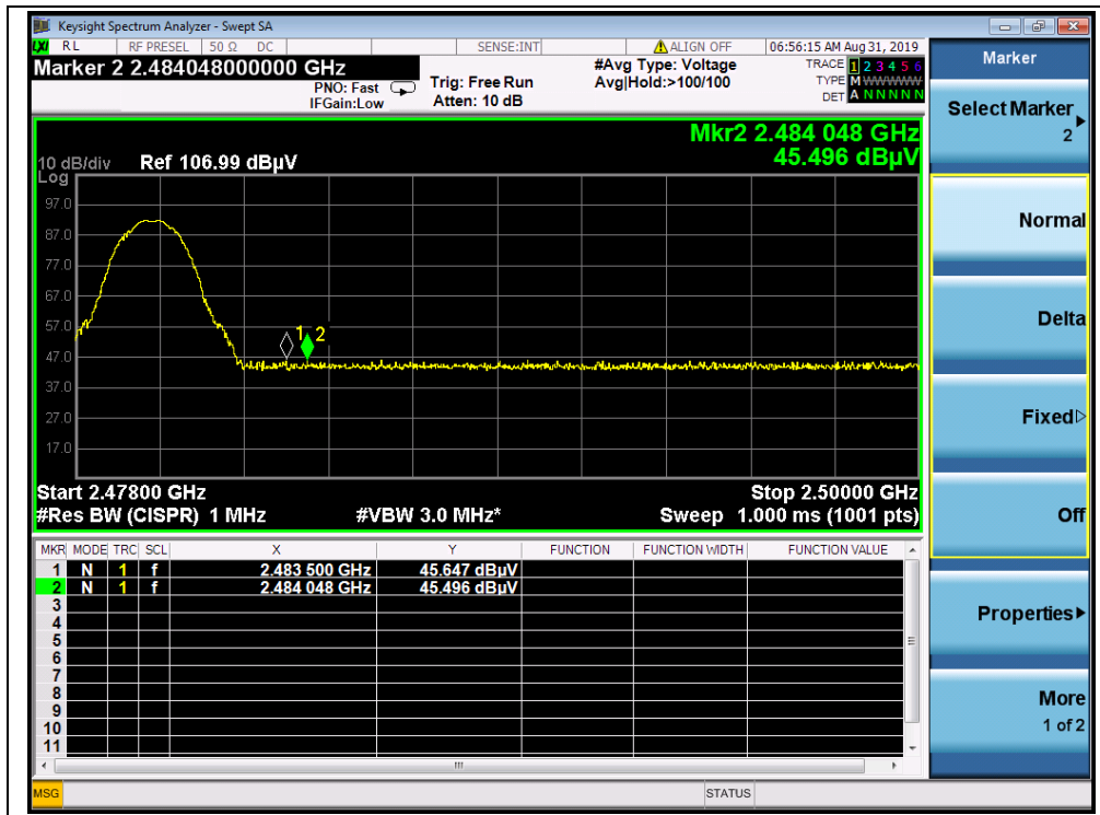
(Channel = 78, AVERAGE, π/4-DQPSK)
