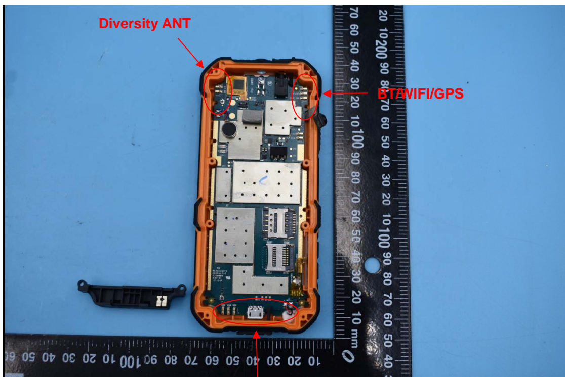
Main ANT
