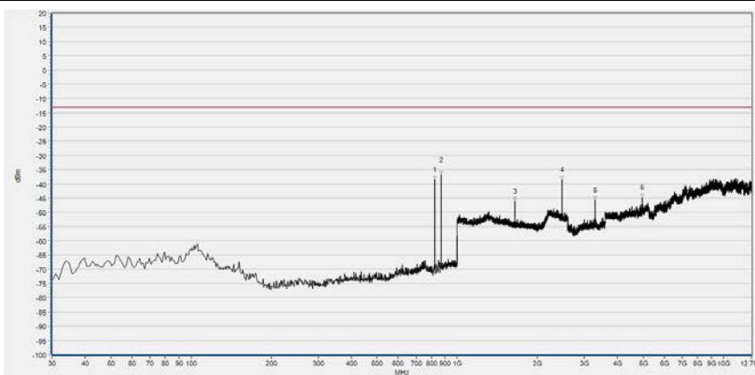
(EDGE 850MHz, Channel = 128, Horizontal)
