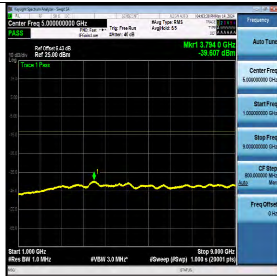
NTNV-N5-PC3-15-5-H-DFT-QPSK-Edge_1RB_Lef t-Ant2-PASS
