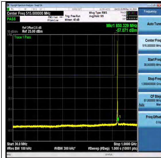
NTNV-N5-PC3-15-5-H-DFT-QPSK-Edge_1RB_Lef t-Ant2-PASS
