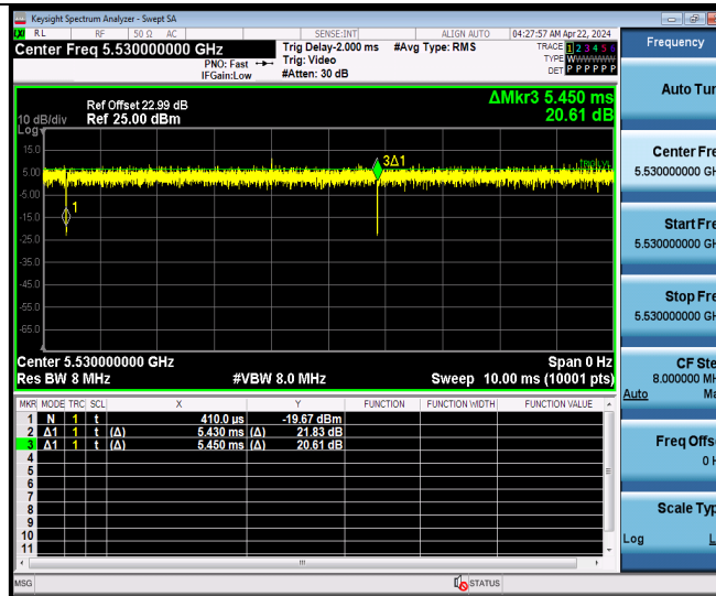
11AC80MIMO Ant9 5530
