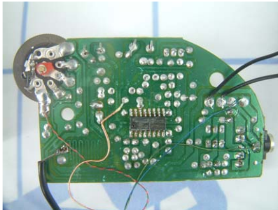
Internal Receiver PCB View-Base
