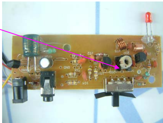
Internal Transmitter PCB View-front
