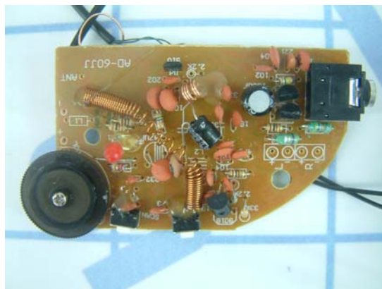
Internal Receiver PCB View-front
