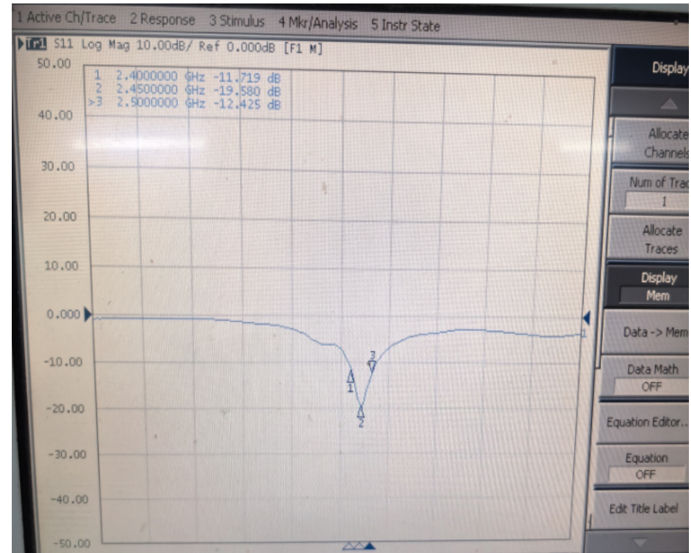
天线回波损耗 Antenna Return loss
