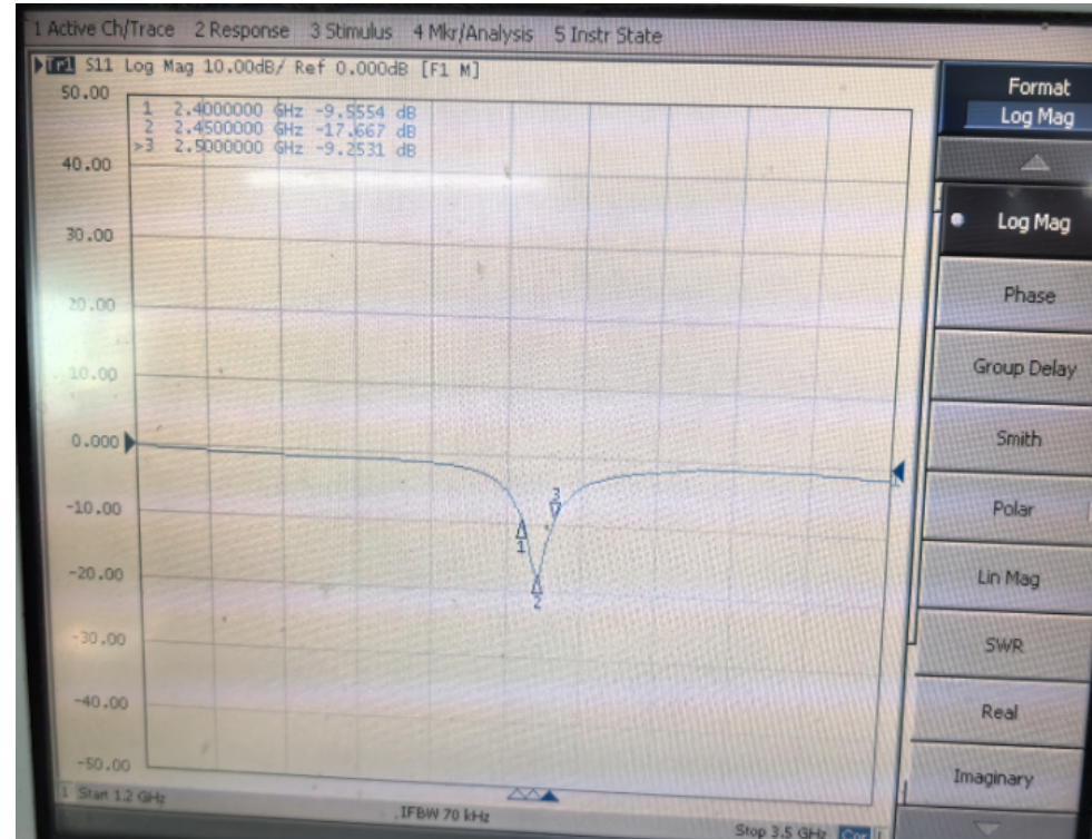
天线回波损耗 Antenna Return loss
