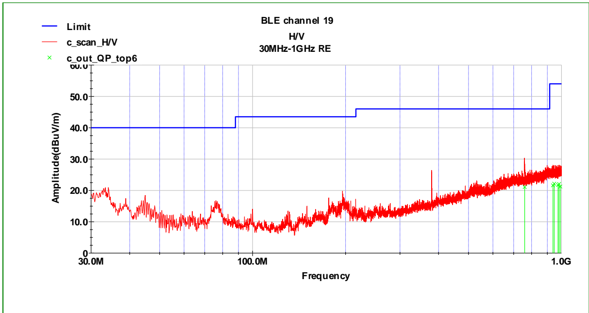
Fig.20 Radiated Emission of channel 19 in 30MHz-1GHz
