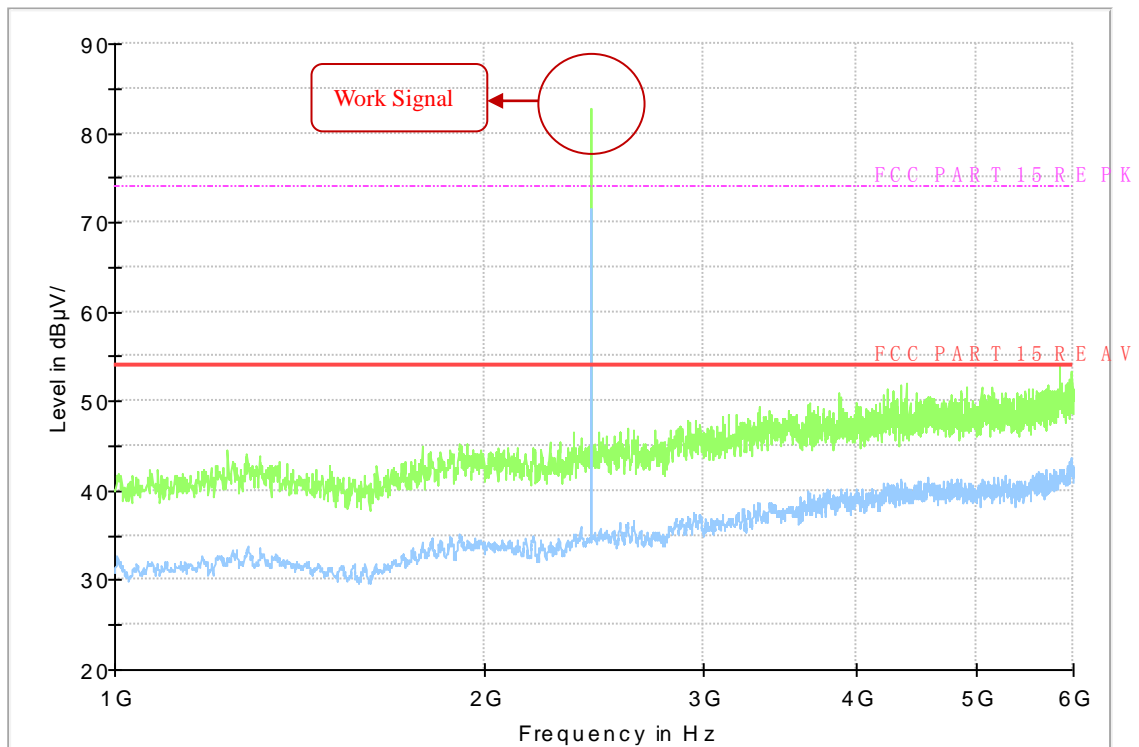
Fig.21 Radiated Emission of channel 19 in 1GHz-6GHz
