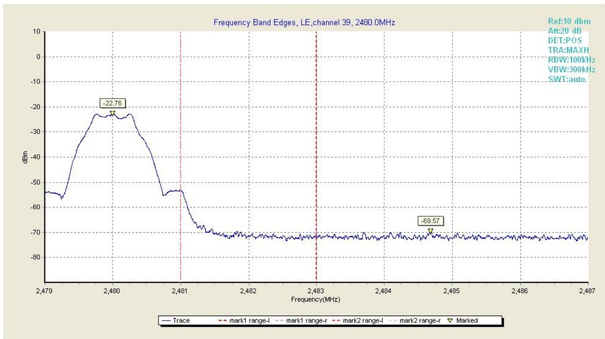
Fig8. Frequency Band Edges in channel 39,2480MHz
