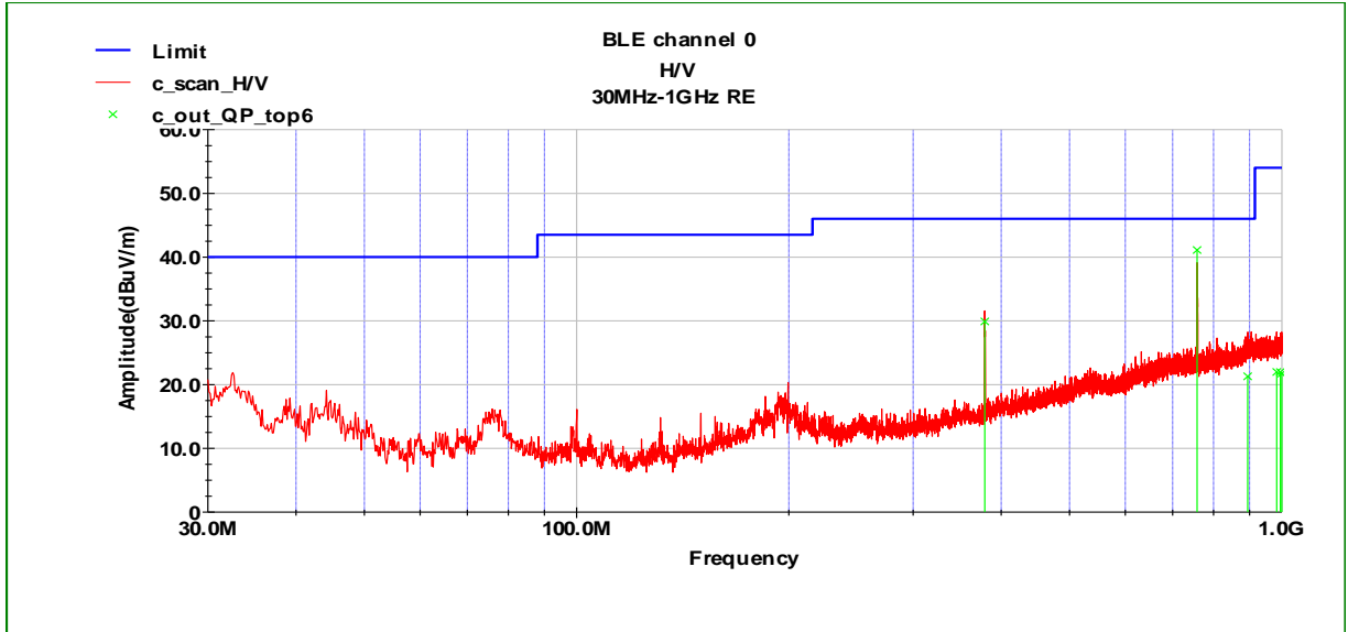
Fig.18 Radiated Emission of channel 0 in 30MHz-1GHz
