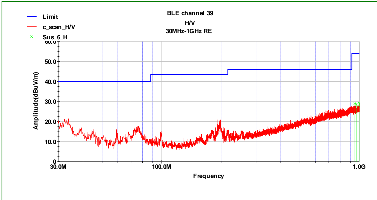
Fig.22 Radiated Emission of channel 39 in 30MHz-1GHz
