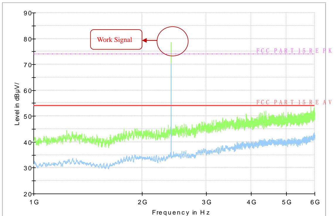
Fig.19 Radiated Emission of channel 0 in 1GHz-6GHz
