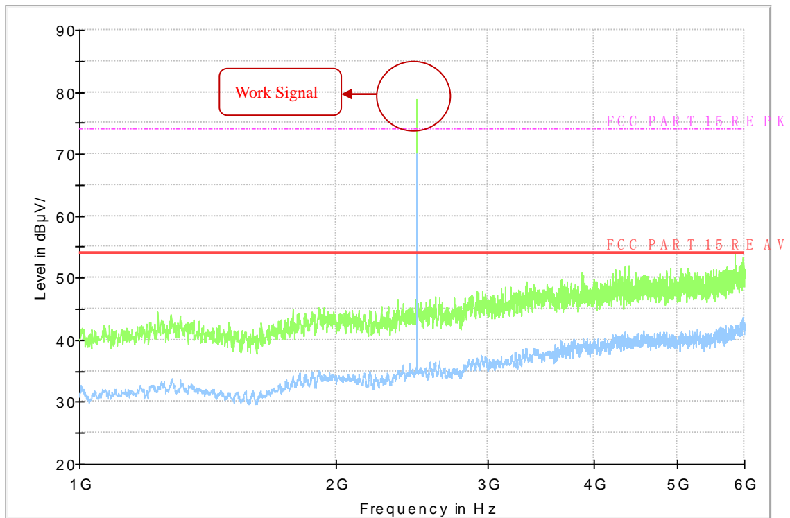
Fig.23 Radiated Emission of channel 39 in 1GHz-6GHz
