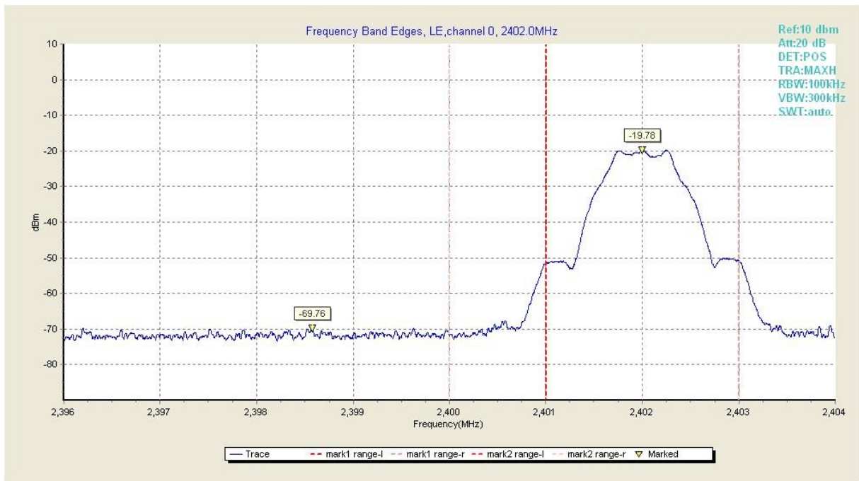
Fig7. Frequency Band Edges in channel 0,2402MHz
