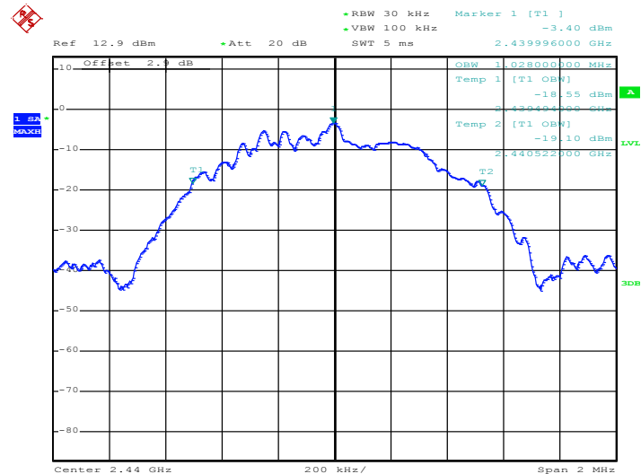
99% Occupied Bandwidth Plot on Channel 19
