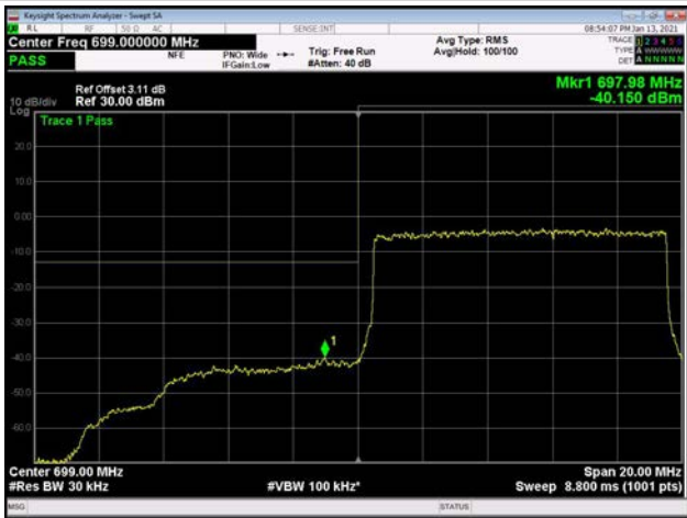
10MHz / 64QAM / Low Channel / 1RB
