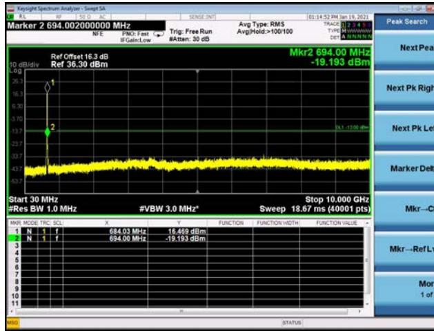
LTE Band 71 _ 15MHz BW _ High Channel
