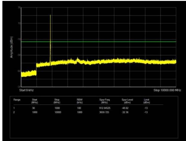
LTE Band 25 _ 15MHz BW _ Low Channel
