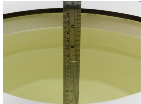
Fig 10.2 Photo of Liquid Height for Body SAR
